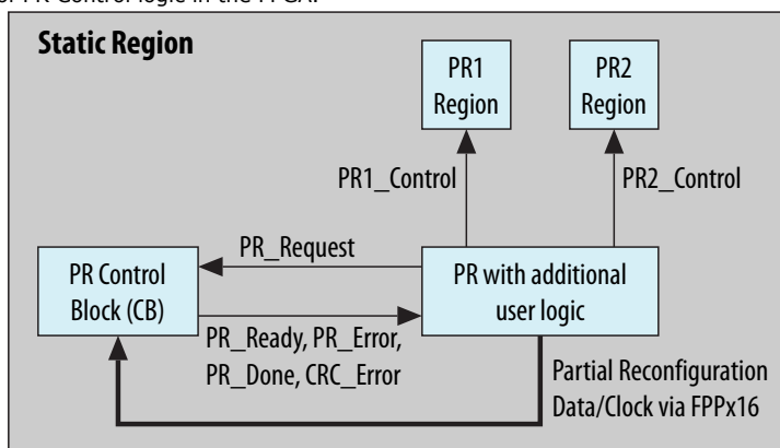
Figure 46. Example of a PR System with Two PR Regions
