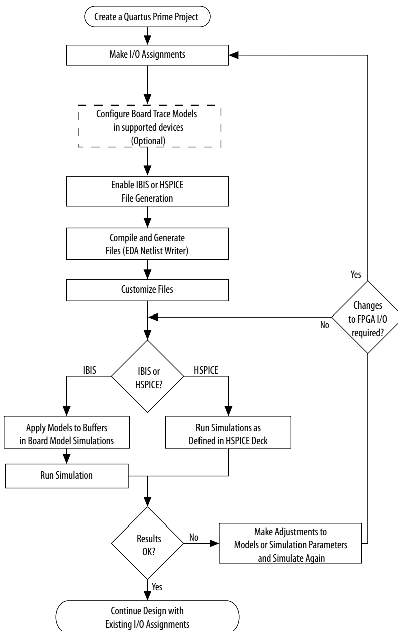
Figure 26. Third-Party Board Signal Integrity Analysis Flow
