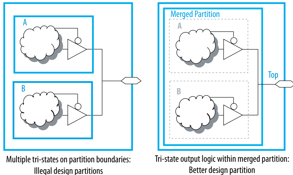
Figure 253. Including All Tri-State Output Logic in the Same Partition
