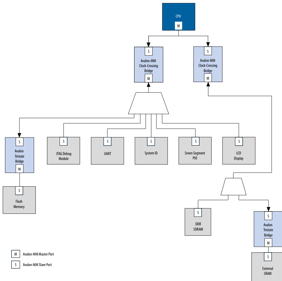
Figure 173. Avalon-MM Clock Crossing Bridge
