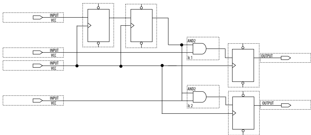
Figure 226. Internally Synchronized Reset
