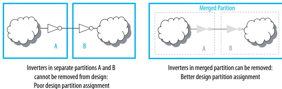
Figure 241. Keeping Logic in the Same Partition for Optimization
