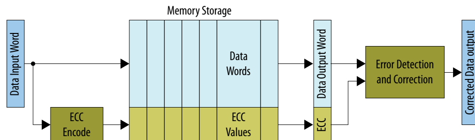
Figure 263. Memory Storage and ECC
