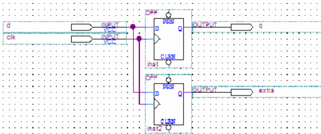
Figure 247. Modified Subdesign with Two Output Registers and Two Output Ports
