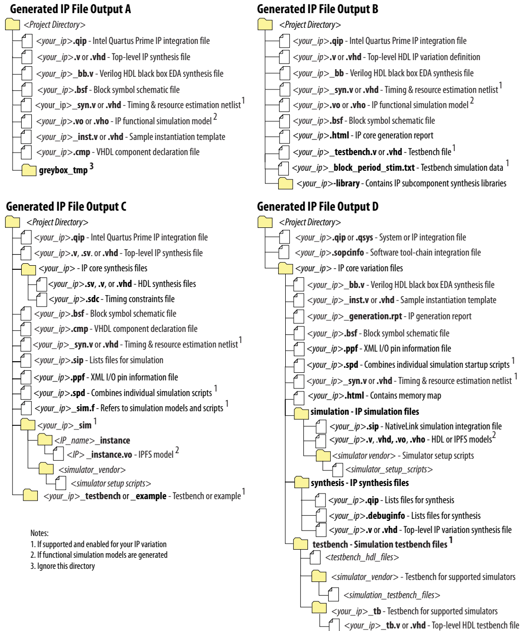
Figure 92. IP Core Generated Files (Legacy Parameter Editors)
