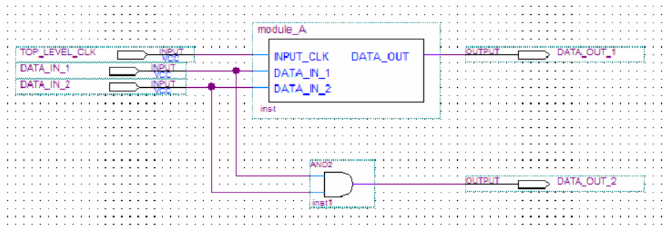
Figure 258. Example Design to Illustrate SDC Constraints
