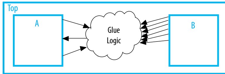
Figure 240. Minimizing I/O between Partitions by Modifying Glue Logic
