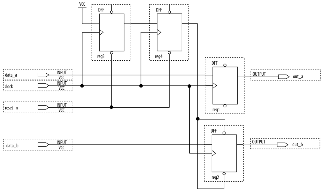
Figure 229. Schematic of Synchronized Asynchronous Reset
