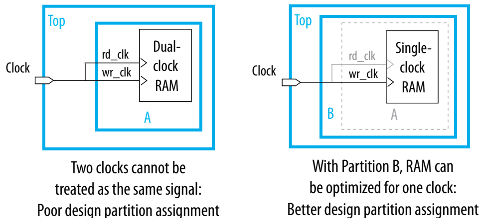
Figure 243. Preventing One Signal from Driving Multiple Partition Inputs
