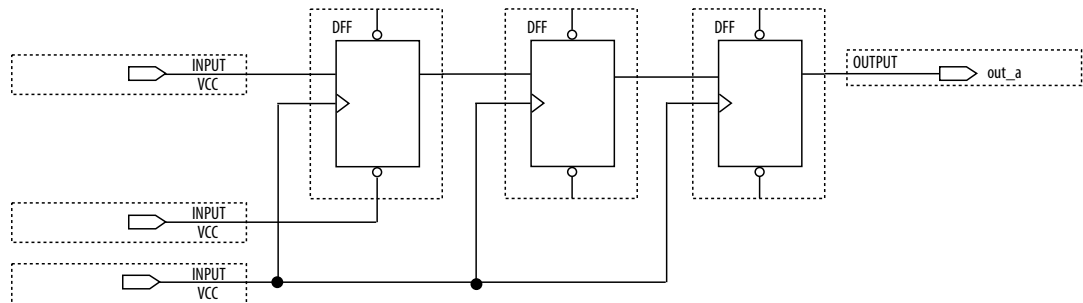
Figure 228. Asynchronous Reset with Follower Registers
