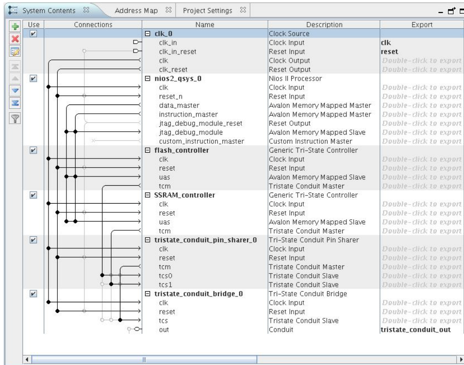
Figure 195. Tri-State Conduit System in Platform Designer (Standard)
