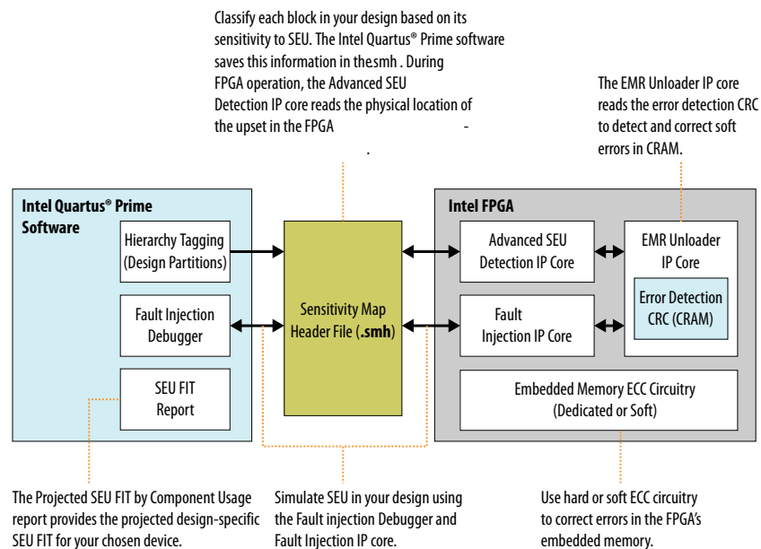
Figure 262. Tools, IP, and Circuitry for Detecting and Correcting SEU
