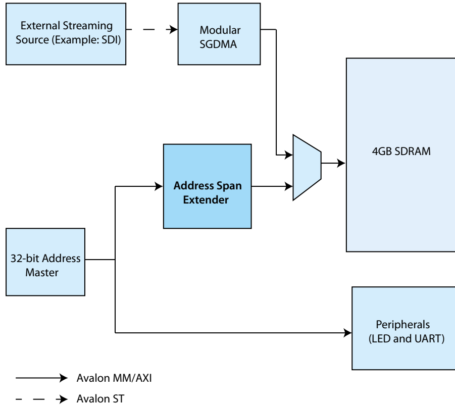
Figure 187. Block Diagram with Address Span Extender
