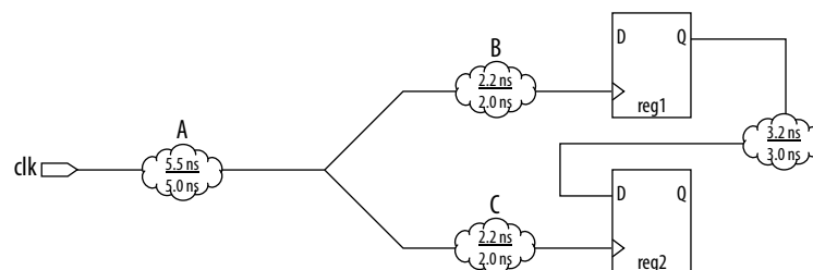
Figure 29. Typical Register to Register Path
