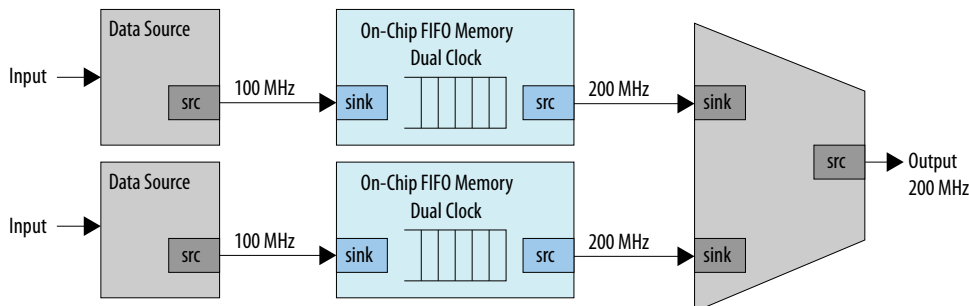
Figure 170. Datapath to Boost the Clock Frequency
