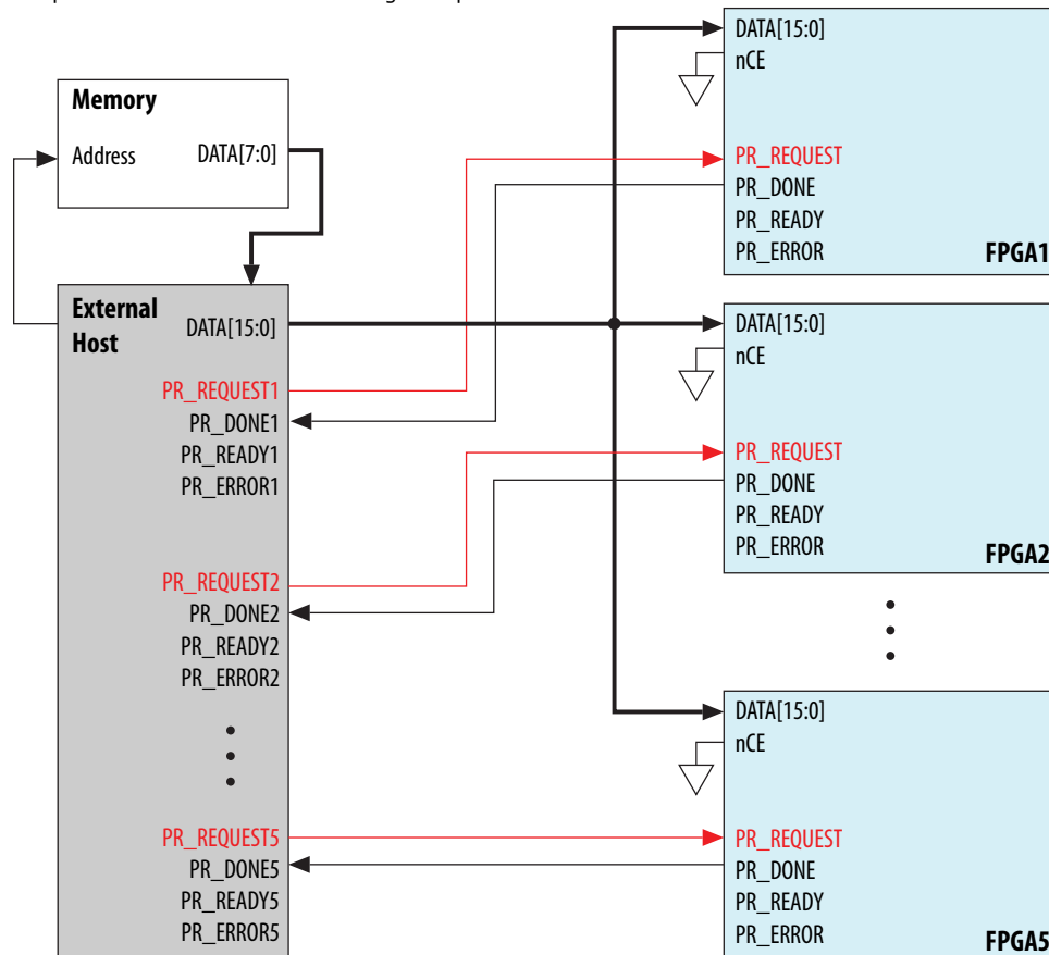
Figure 49. Connecting Multiple FPGAs to an External Host
