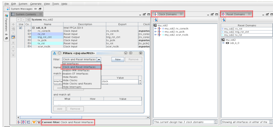
Figure 82. Platform Designer (Standard) Clock and Reset Domains
