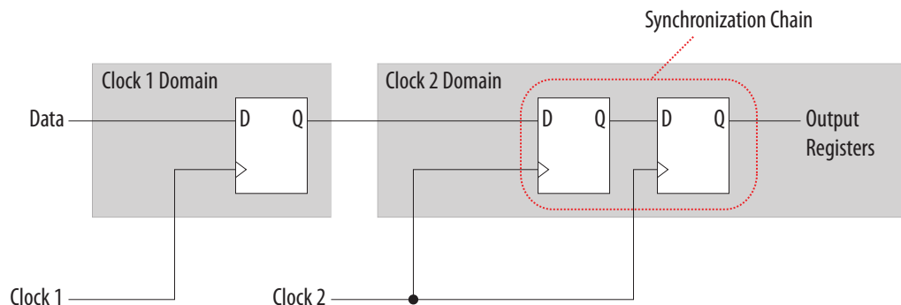
Figure 235. Sample Synchronization Register Chain
