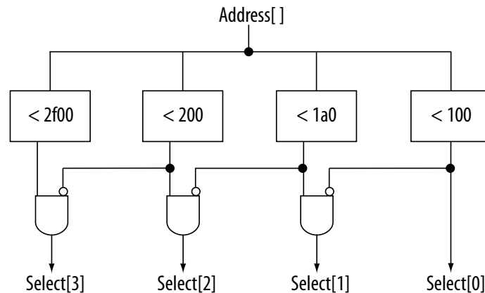
Figure 234. Example Logic Structure for Using Comparators to Check a Bus Value Range
