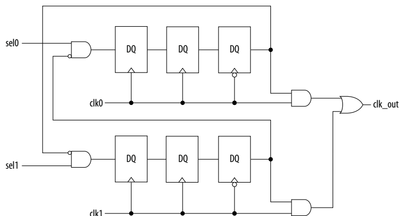
Figure 232. Glitch-Free Clock Multiplexer Structure
