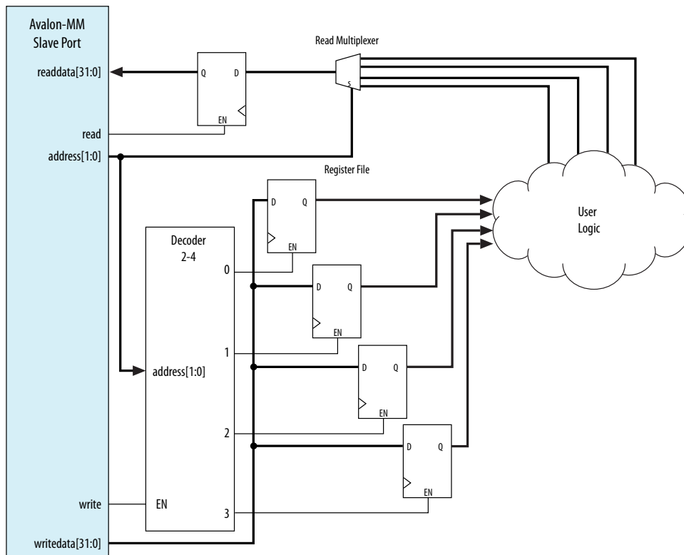
Figure 135. Control and Status Registers (CSR) in a Slave Component
