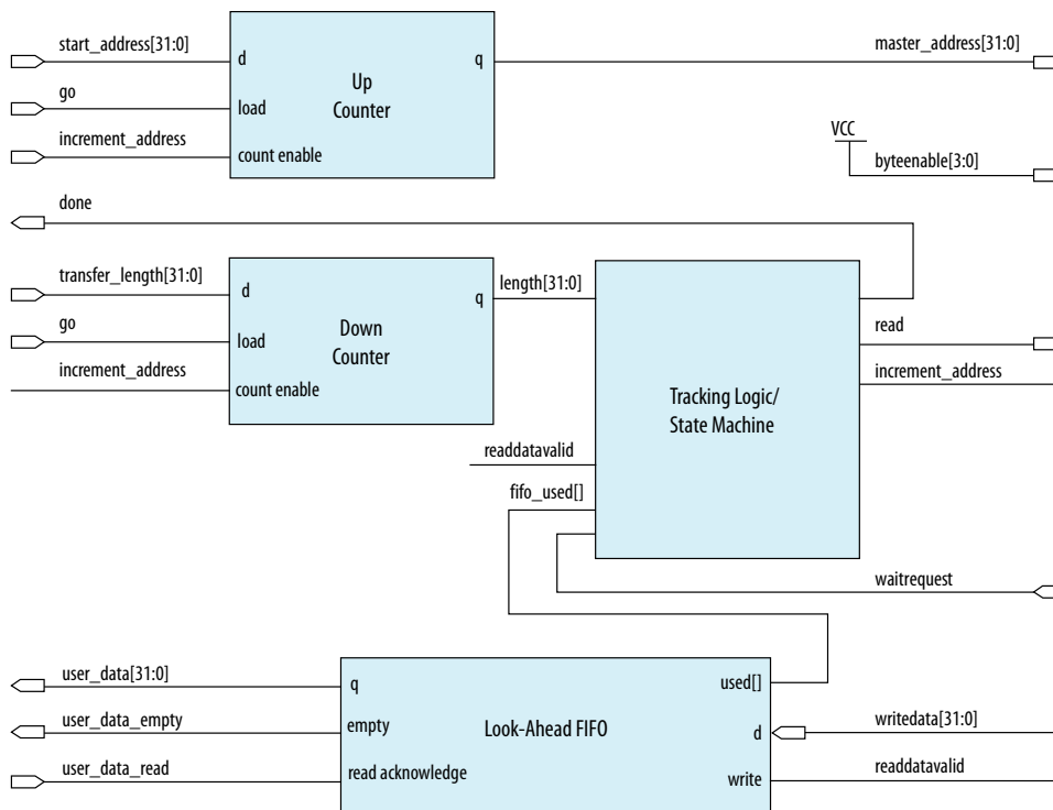
Figure 167. Pipelined Read Master
