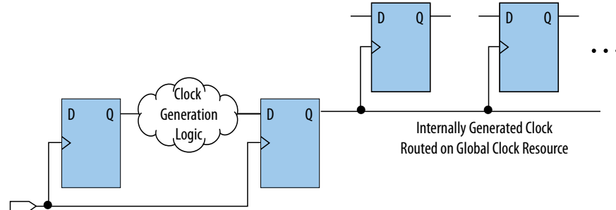
Figure 213. Recommended Clock-Generation Technique
