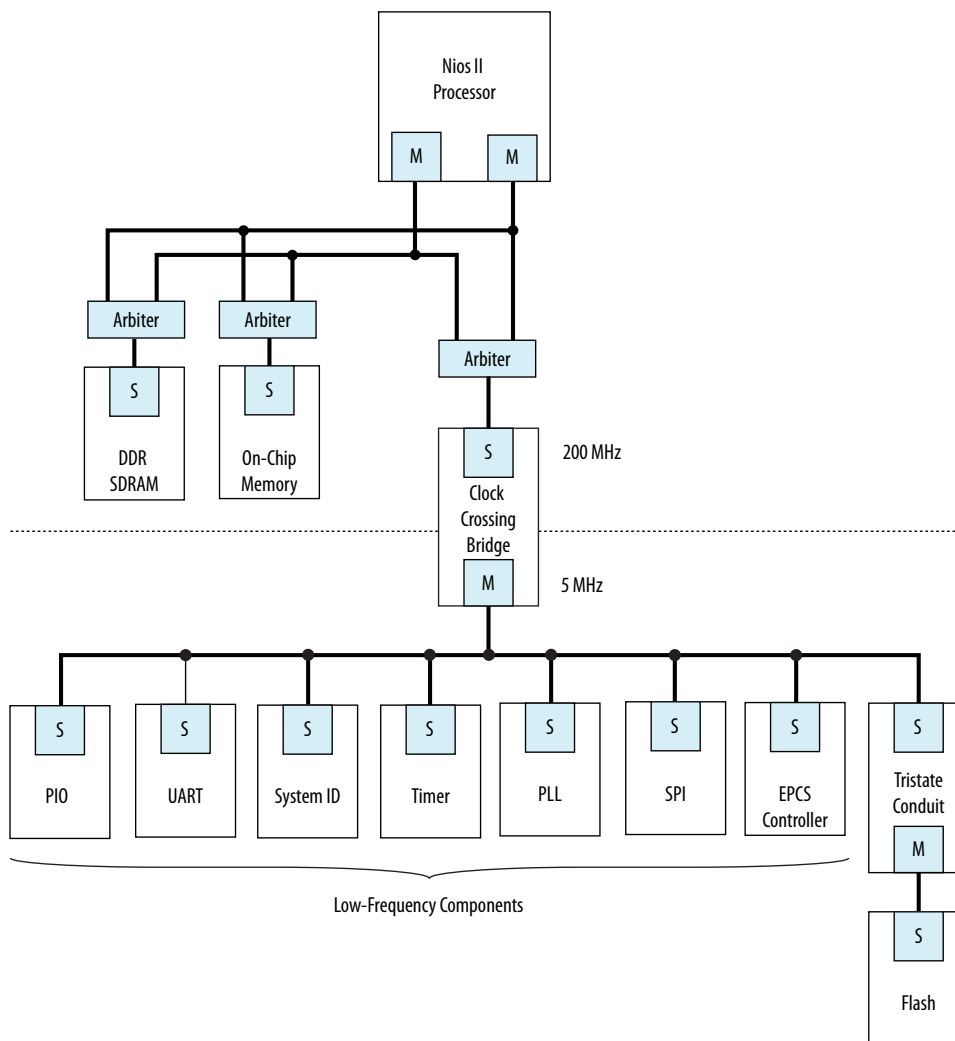
Figure 159. Reducing Power Utilization Using a Bridge to Separate Clock Domains
