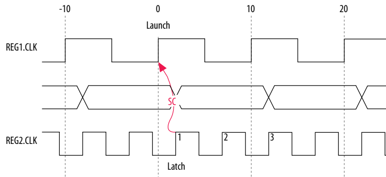
Figure 89. Setup Timing Diagram
