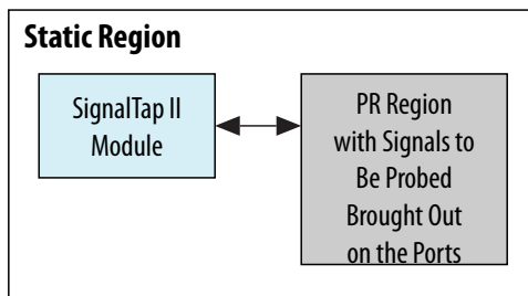
Figure 54. Using Signal Tap with a PR Design
