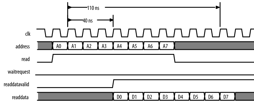
Figure 148. Performance of a Nios II Processor and Memory Operating at 100 MHz
