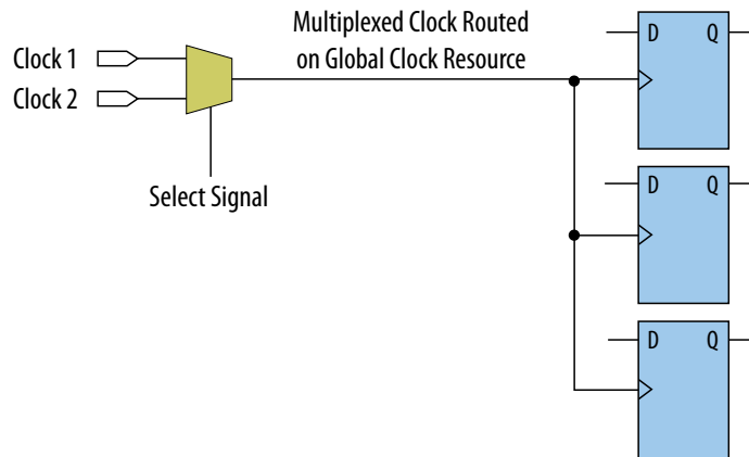
Figure 214. Multiplexing Logic and Clock Sources
