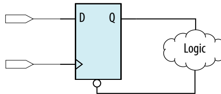
Figure 210. Combinational Loop Through Asynchronous Control Pin
