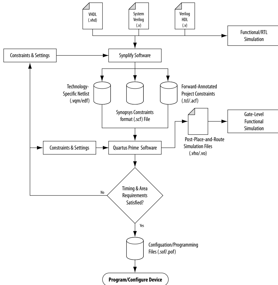
Figure 283. Recommended Design Flow
