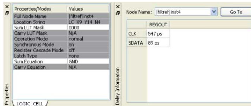
Figure 118. LE Properties in the Resource Property Editor
