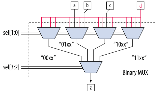
Figure 233. Priority Multiplexer Implementation of an IF Statement
