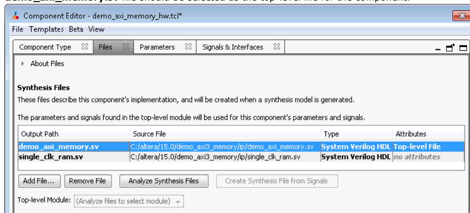
Figure 96. Using HDL Files to Define a Component
