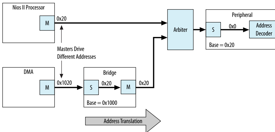
Figure 153. Slaves at Different Addresses and Complicating the System
