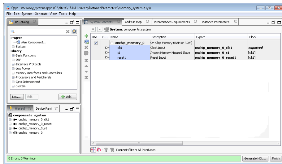
Figure 76. On-Chip Memory Component System and Instance Parameters ( memory_system.qsys )
