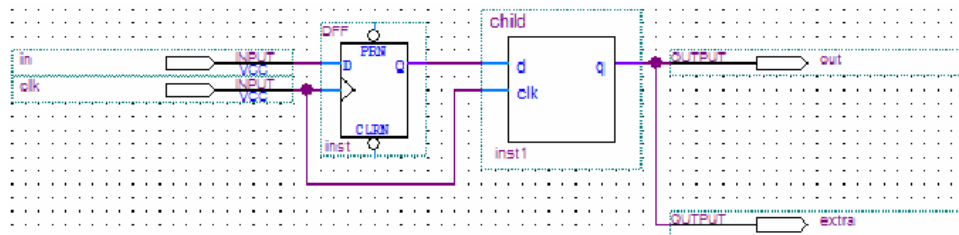
Figure 246. Top-Level Design Instantiating the Subdesign with Two Output Pins
