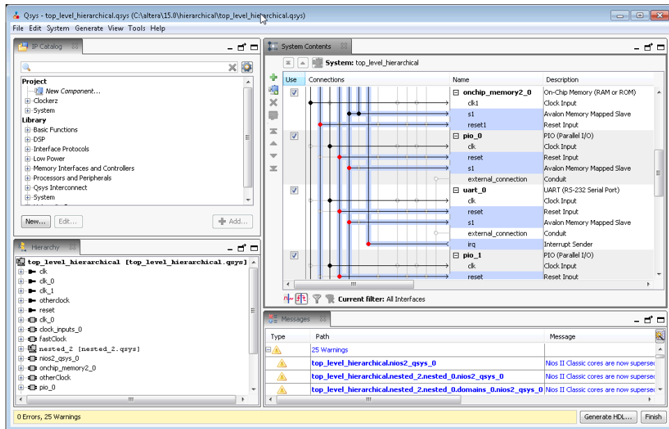
Figure 63. View Your Platform Designer (Standard) System
