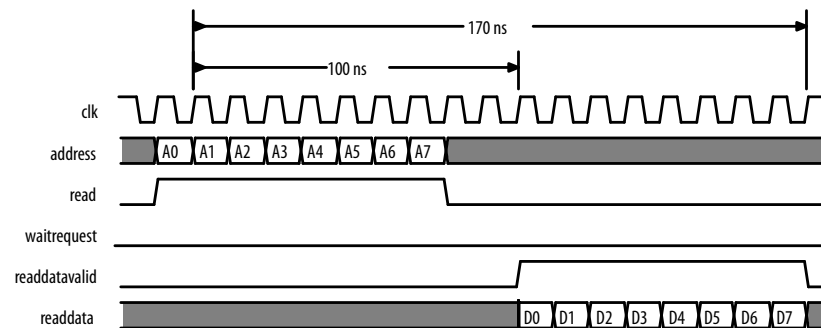
Figure 149. Performance of a Nios II Processor and Eight Reads with Ten Cycles Latency
