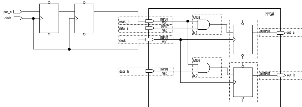
Figure 225. Externally Synchronized Reset
