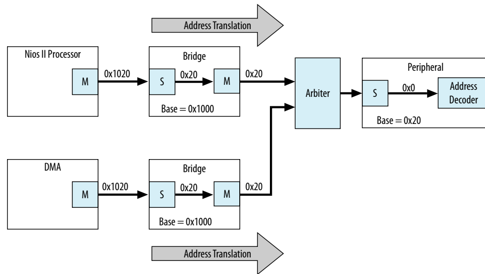
Figure 154. Address Translation Corrected With Bridge
