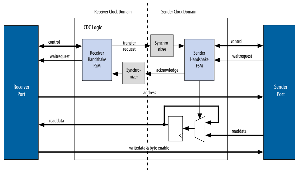
Figure 158. Clock Crossing Adapter
