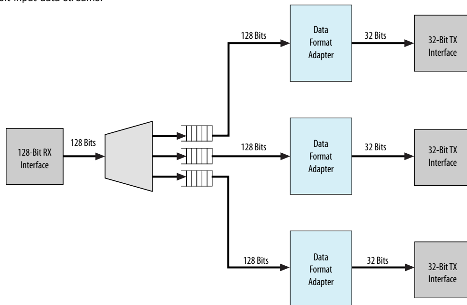
Figure 124. Avalon Streaming Interconnect with Data Format Adapter
