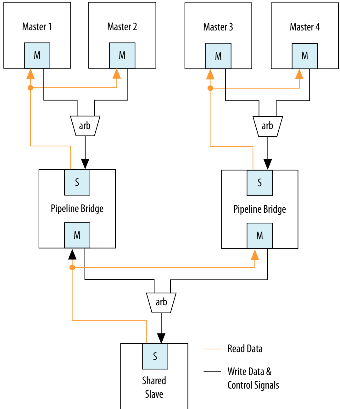
Figure 144. Tree of Bridges
