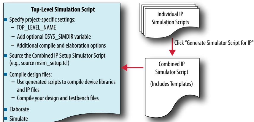
Figure 21. Incorporating Generated Simulator Setup Scripts into a Top-Level Simulation Script
