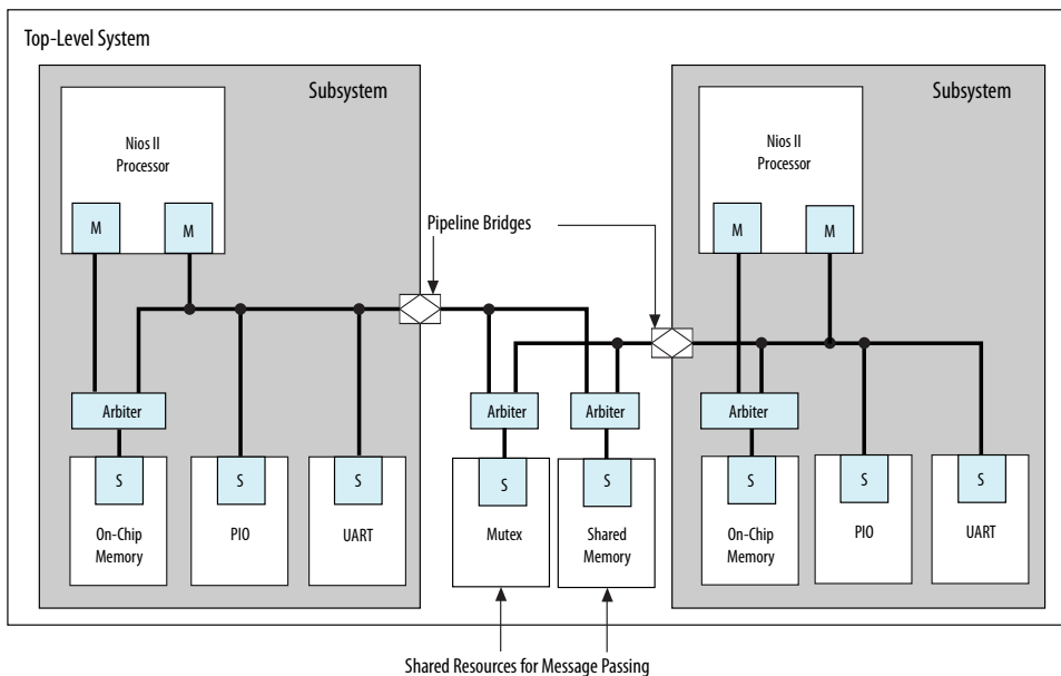
Figure 137. Passing Messages Between Subsystems
