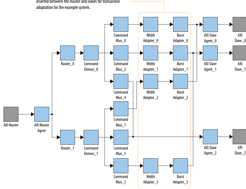
Figure 179. AXI System Without a Bridge
