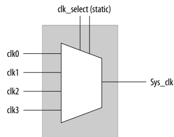
Figure 231. Simple Clock Multiplexer in a 6-Input LUT
