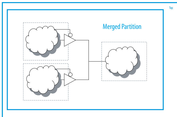
Figure 252. Merged Partition Allows Synthesis to Convert Internal Tri-State Logic to Combinational Logic
