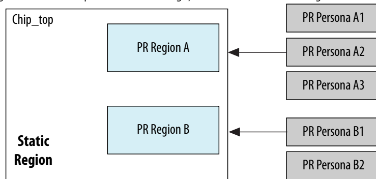
Figure 36. Partial Reconfiguration Project Structure
