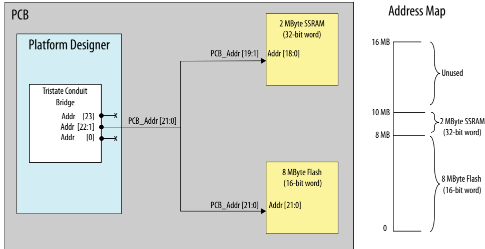
Figure 194. Address Connections from Platform Designer (Standard) System to PCB
