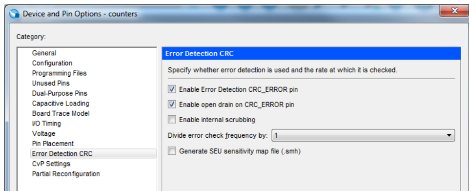
Figure 269. Device and Pin Options Error Detection CRC Tab
