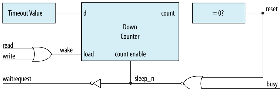
Figure 161. Hardware-Controlled Sleep Components
