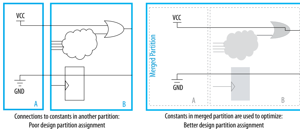
Figure 242. Keeping Constants in the Same Partition as the Logic They Feed
