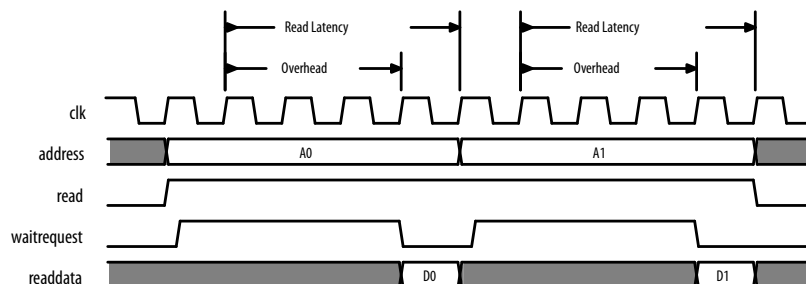
Figure 146. Low-Efficiency Read Transfer
