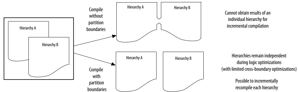
Figure 237. Effects of Partition Boundaries During Logic Optimization
