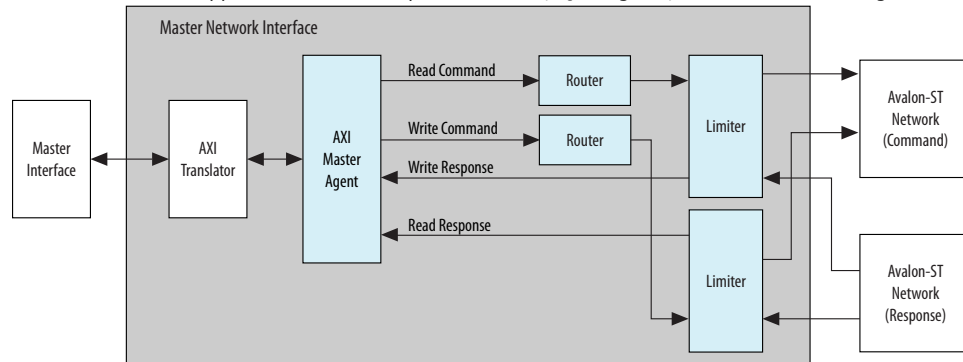
Figure 108. AXI Master Network Interface
