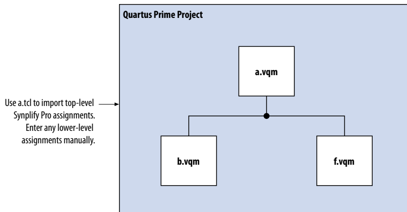
Figure 289. Design Flow Using Multiple .vqm Files with One Intel Quartus Prime Project
