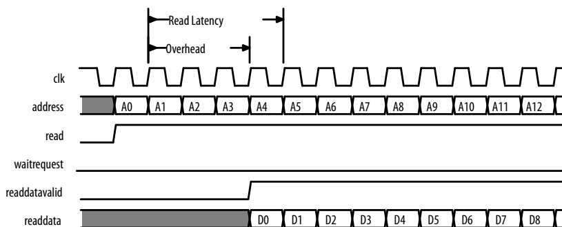
Figure 147. High Efficiency Read Transfer
