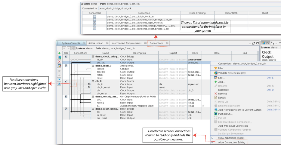
Figure 61. Connections Column in the System Contents Tab
