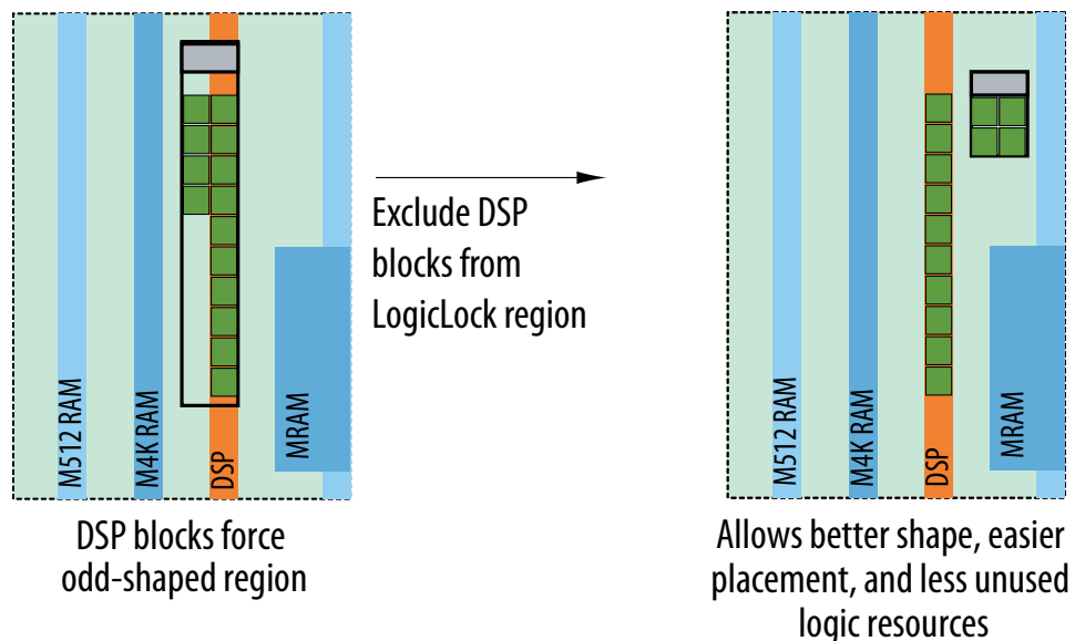
Figure 261. LogicLock Resource Exclusion Example
