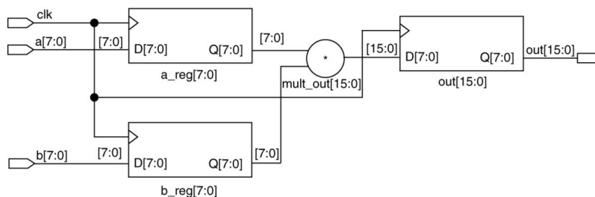
Figure 284. HDL Analyst View of LPM_MULT IP Core (Unsigned 8x8 Multiplier with Pipeline=2)
