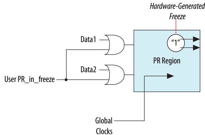
Figure 43. Freezing at PR Region Boundary
