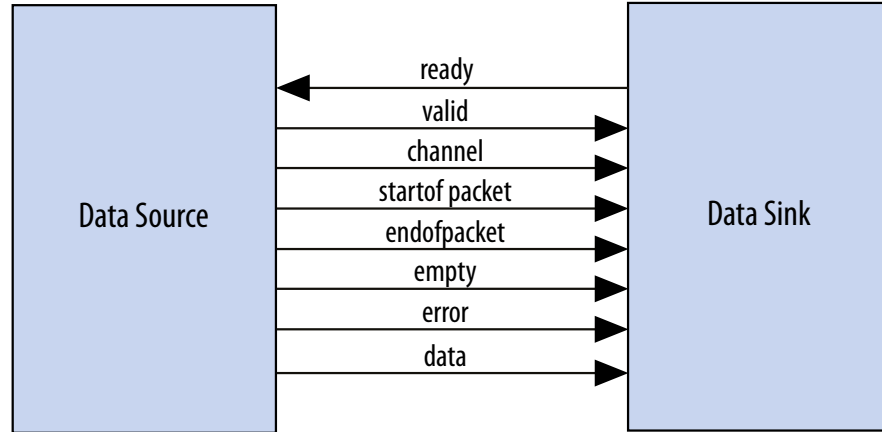
Figure 123. Signals Indicating the Start and End of Packets, Channel Numbers, Error Conditions, and Backpressure
