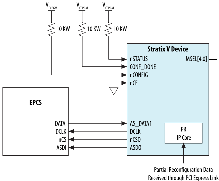
Figure 50. Connecting to an Internal Host
