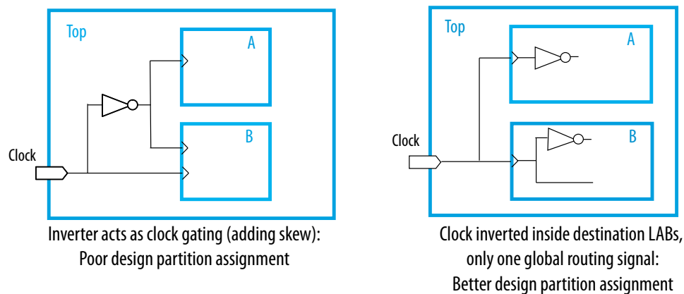
Figure 244. Inverting Clock Signal in Destination Partitions
