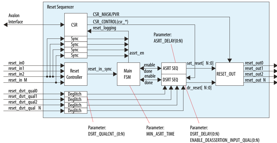
Figure 128. Elements and Flow of a Reset Sequencer
