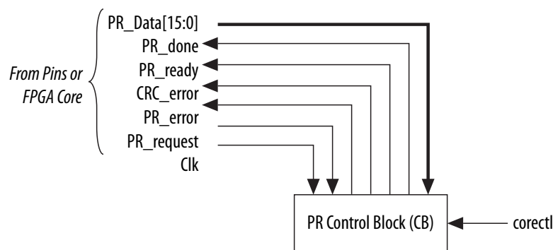
Figure 45. Partial Reconfiguration Interface Signals
