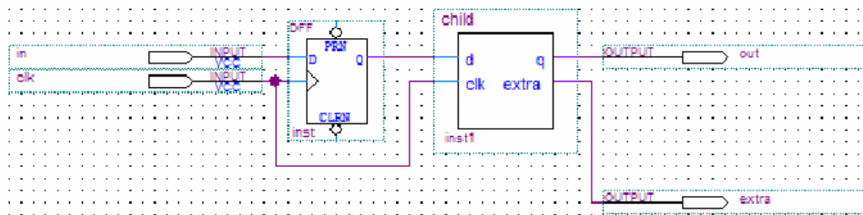
Figure 248. Modified Top-Level Design Connecting Two Output Ports to Output Pins
