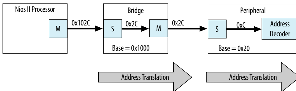
Figure 152. Bridge Address Translation
