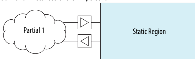
Figure 42. Wire-LUTs at PR Region Boundary
