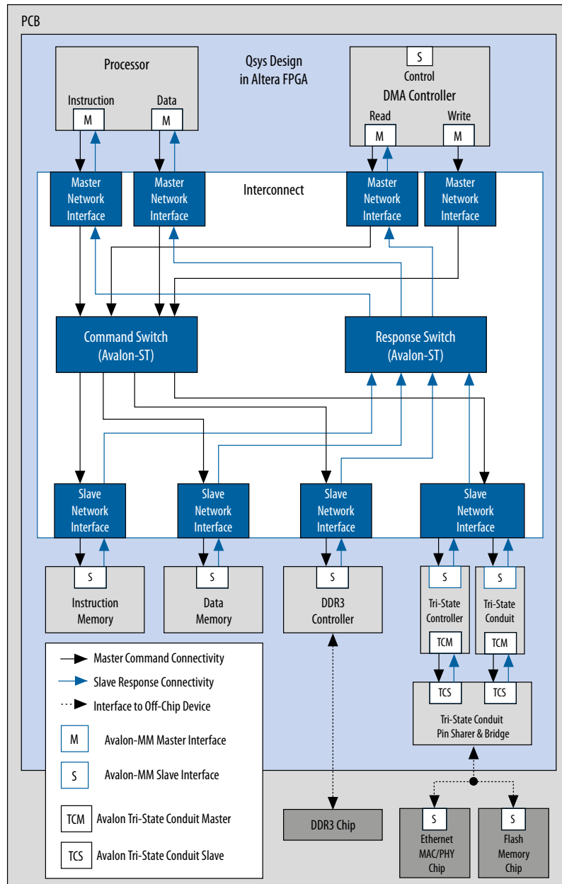
Figure 103. Platform Designer (Standard) interconnect for an Avalon-MM System with Multiple Masters
