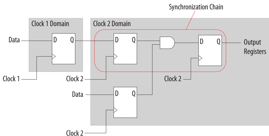
Figure 236. Sample Synchronization Register Chain Containing Logic
