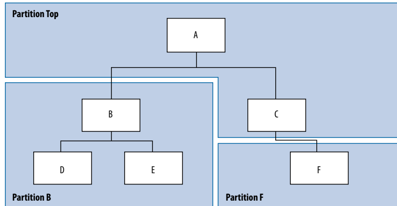
Figure 292. Partitions in a Hierarchical Design
