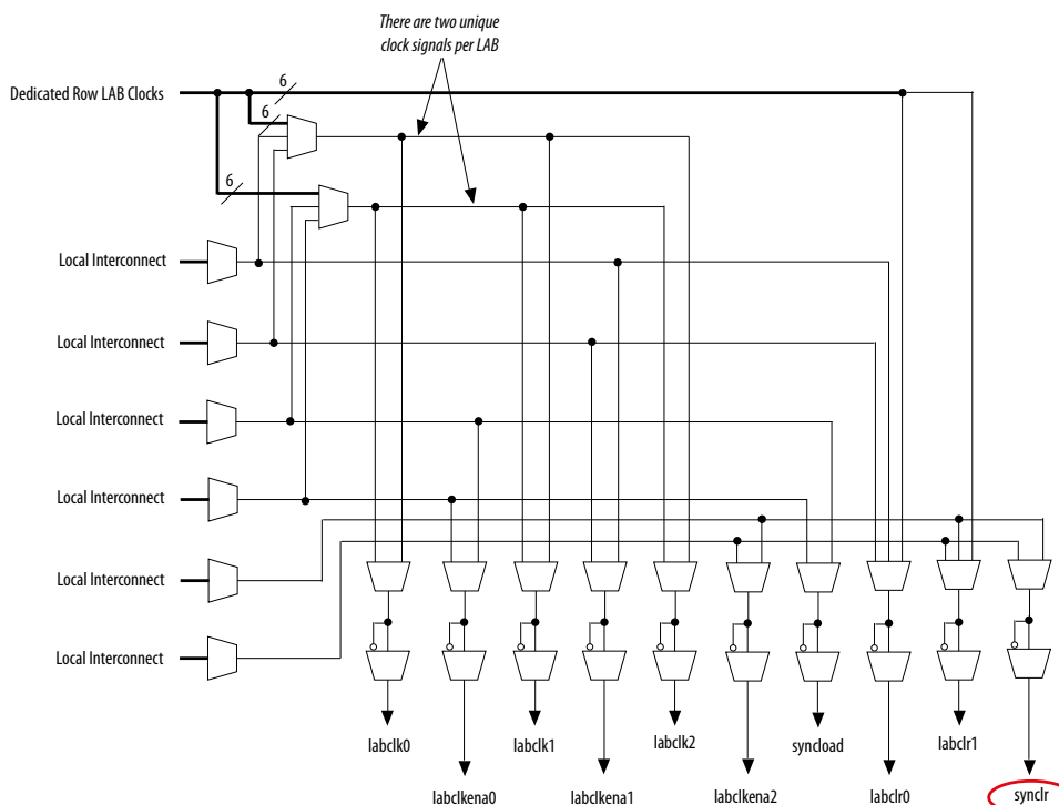
Figure 224. LAB-Wide Control Signals
