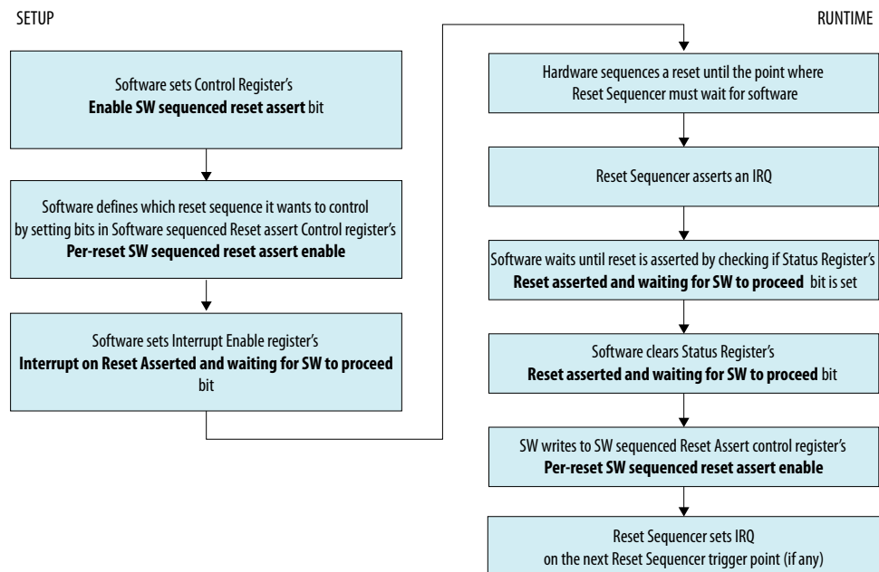
Figure 132. Reset Assert (Software Sequenced) Flow
