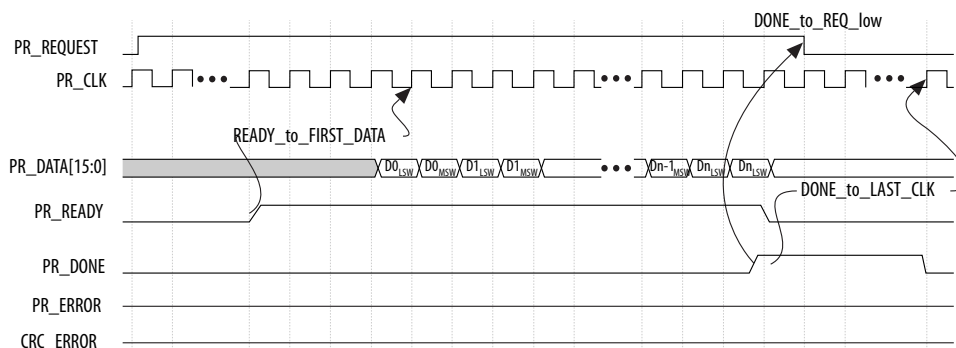
Figure 47. Partial Reconfiguration Timing Diagram
