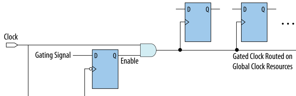
Figure 216. Recommended Clock-Gating Technique for Clock Active on Rising Edge
