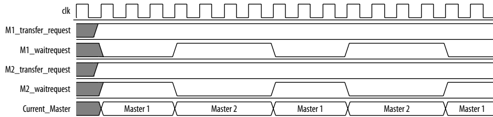
Figure 114. Arbitration of Two Masters with a Gap in Transfer Requests
