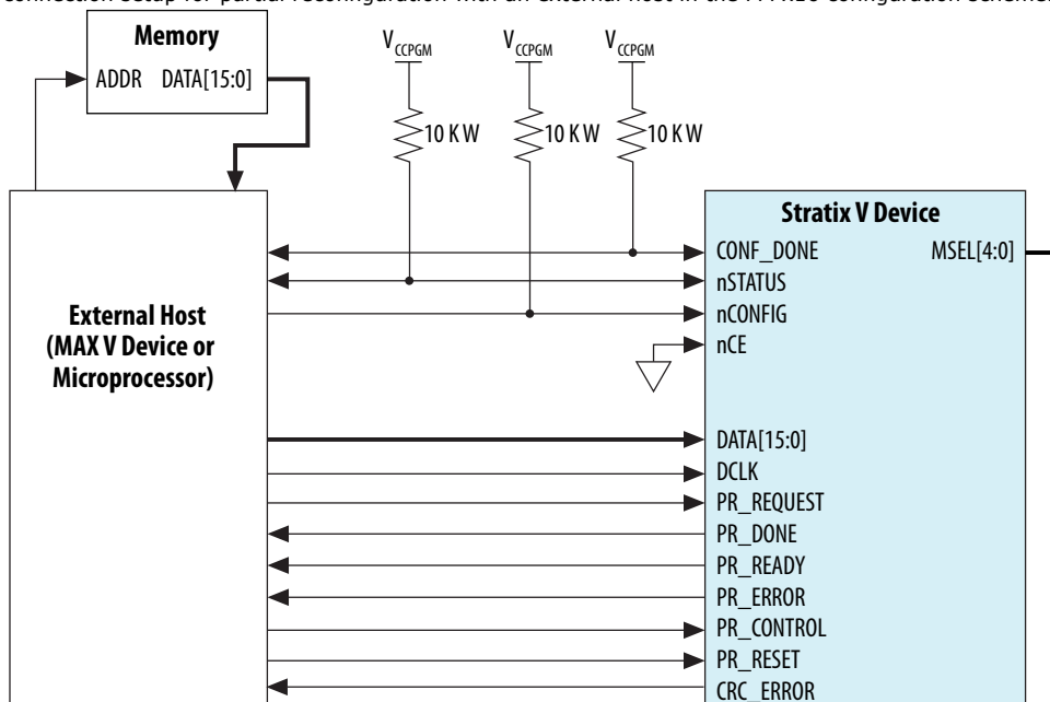
Figure 48. Connecting to an External Host
