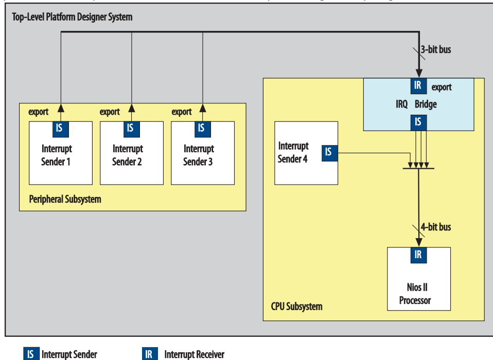
Figure 126. Platform Designer (Standard) IRQ Bridge Application
