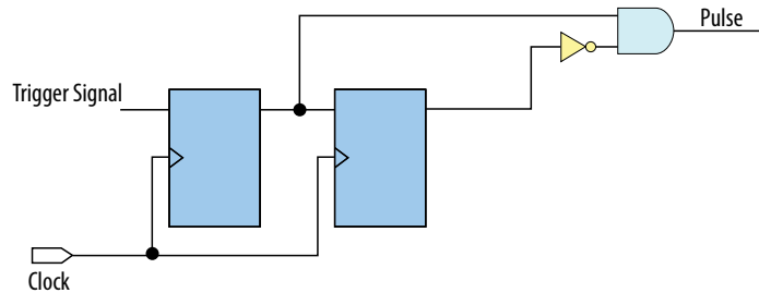
Figure 212. Recommended Synchronous Pulse-Generation Technique
