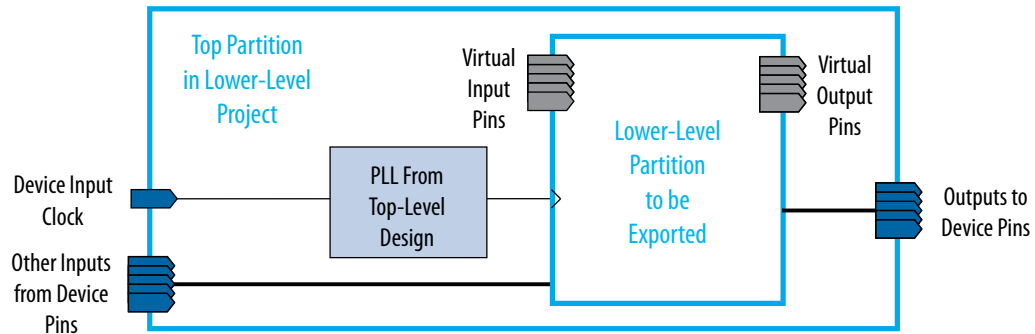
Figure 255. Recreating a Top-Level PLL in a Lower-Level Partition
