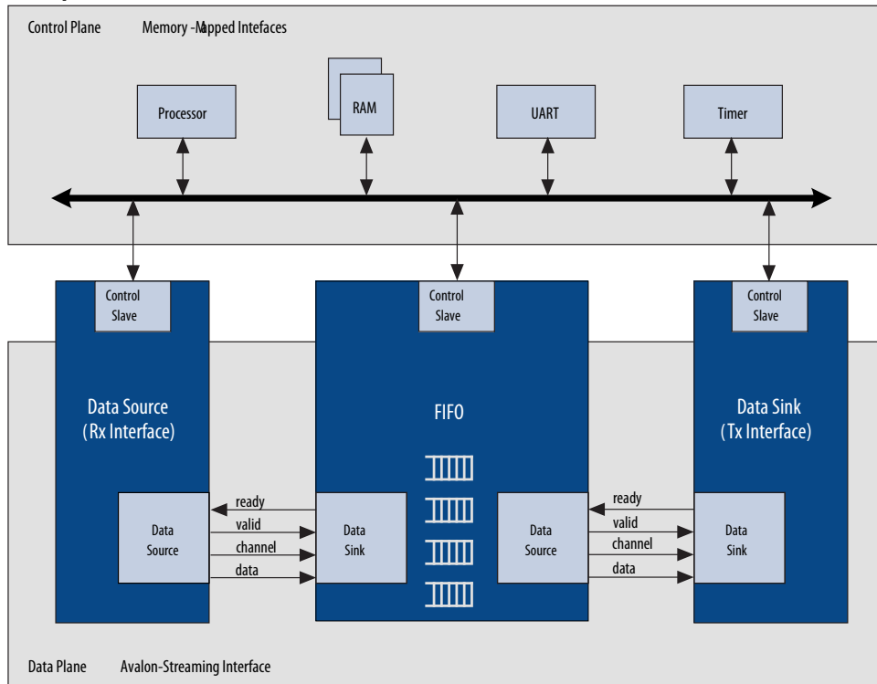
Figure 122. Avalon-ST Connection Between the Source and Sink
