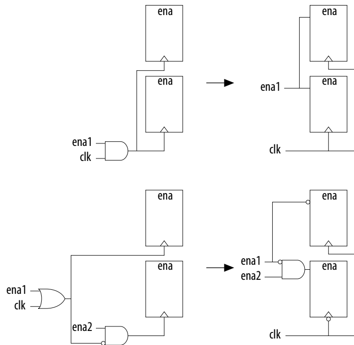
Figure 272. Example Gated Clock Conversion
