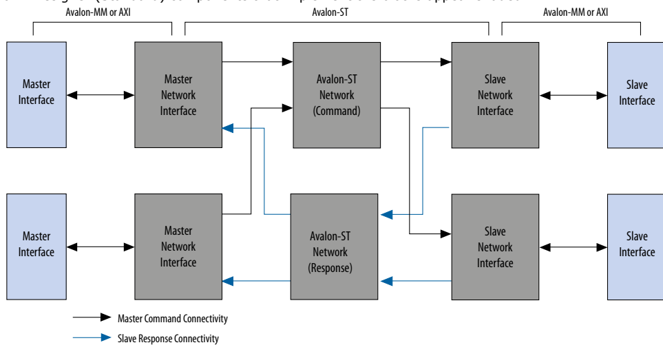
Figure 104. Transformation when Generating a System with Memory-Mapped and Slave Components
