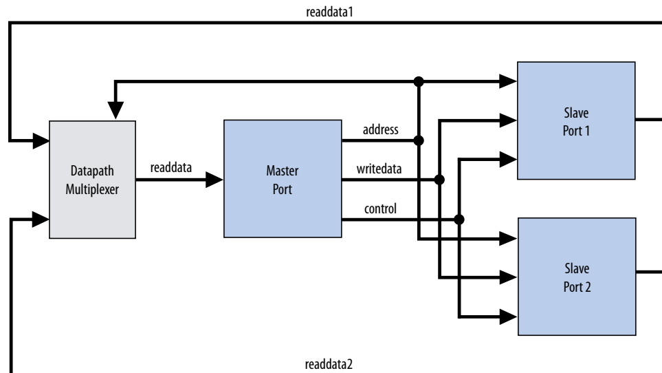
Figure 117. Datapath Multiplexing Logic for One Master and Two Slaves
