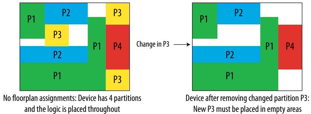
Figure 259. Representation of Device Floorplan without Location Assignments
