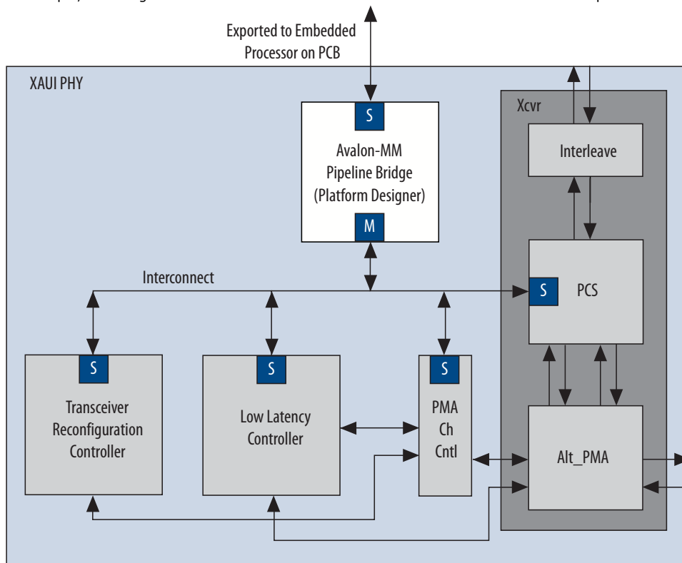
Figure 174. Avalon-MM Pipeline Bridge in a XAUI PHY Transceiver IP Core
