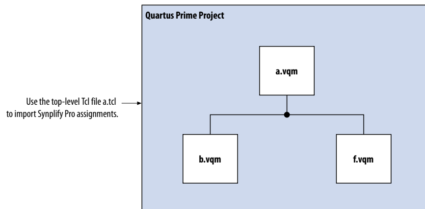
Figure 286. Design Flow Using Multiple .vqm Files with One Intel Quartus Prime Project
