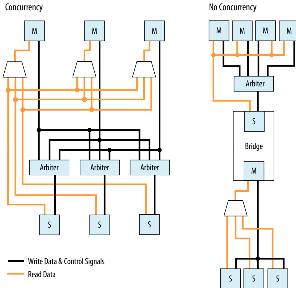
Figure 145. Differences Between Systems With and Without a Pipeline Bridge
