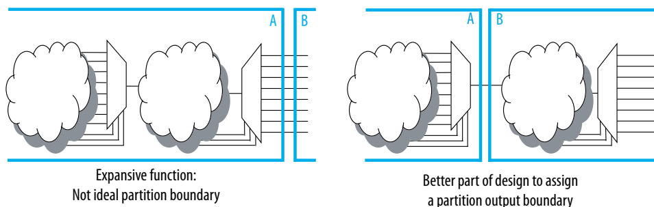
Figure 239. Minimizing I/O Between Partitions by Moving the Partition Boundary
