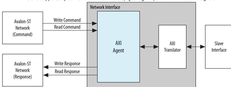
Figure 110. AXI Slave Network Interface
