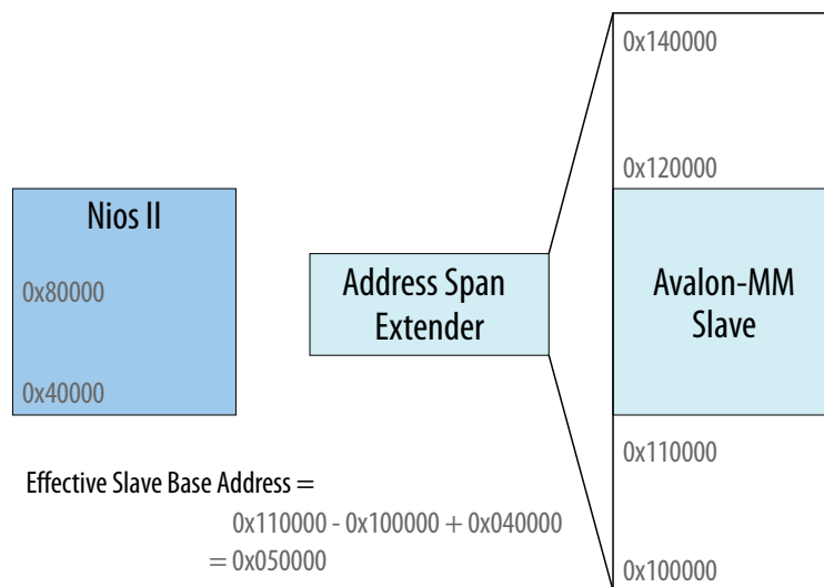
Figure 190. Nios II Support and the Address Span Extender
