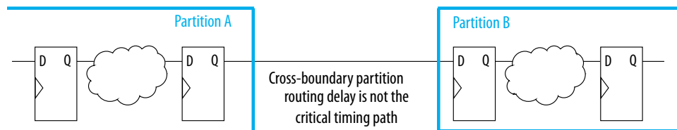
Figure 238. Registering Partition I/O
