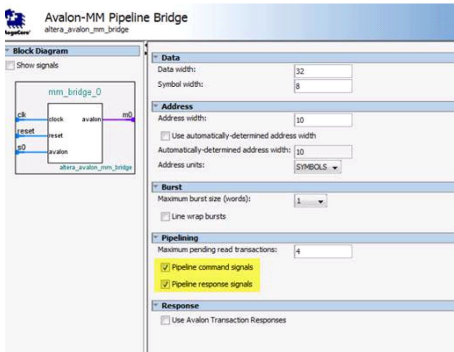
Figure 136. Avalon-MM Pipeline Bridge
