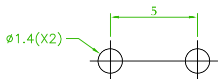
MOUNTING HOLE
