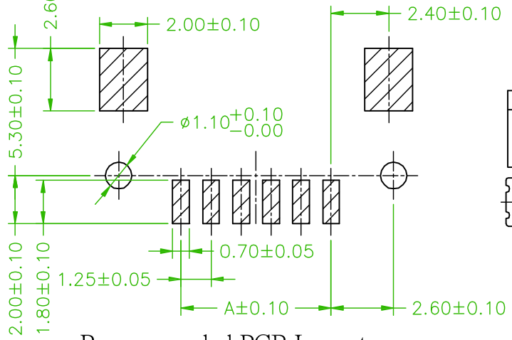
Recommended PCB Layout (PCB TOLERANCE ±0.05)
