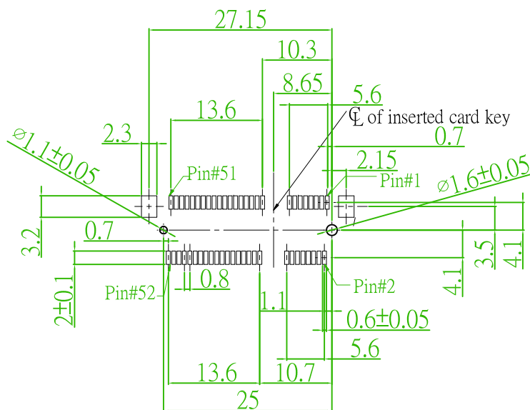
PCB LAYOUT : COMPONENT SIDE ±0.1
