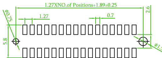
Outer Peg
