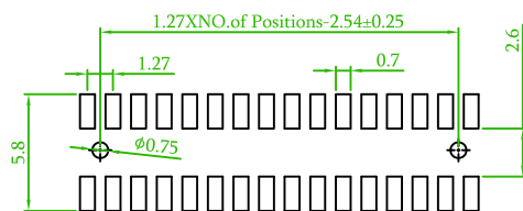
Inner Peg
