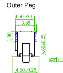
Outer Peg
