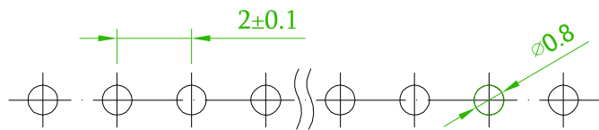
Recommended PCB Layout (PCB TOLERANCE ±0.05)
