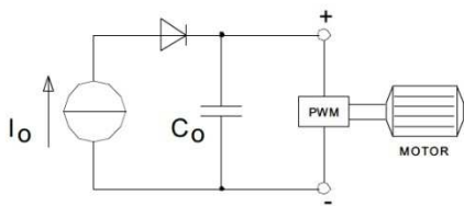
Conventional power supply: braking power charges output capacitor C_o
