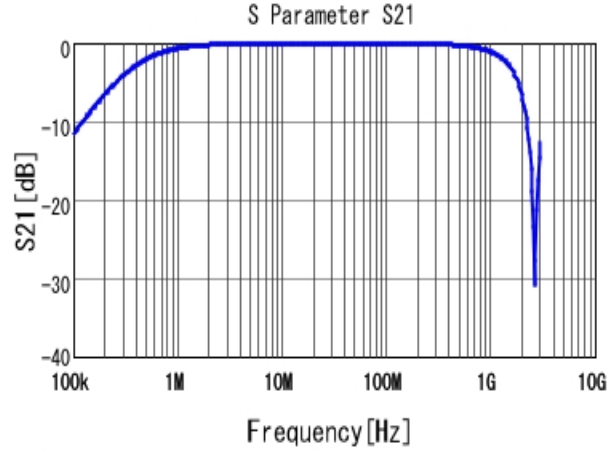
■ DE2E3KY472MN3AM02F S21 DCOV, 20degC
