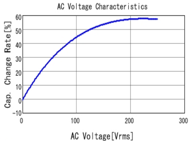
■ DE2E3KY472MN3AM02F C-AC Voltage capchange, DCOV, 20.0
