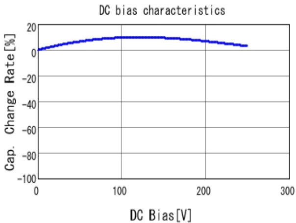
■ DE2E3KY472MN3AM02F C-DC bias capchange, 20.0degC, AC1
