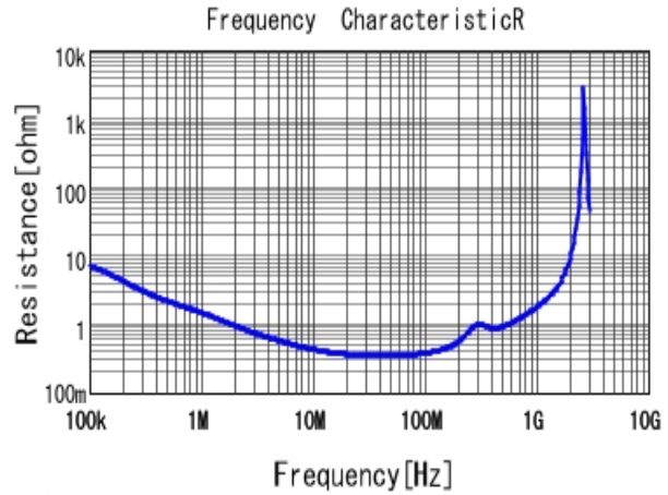
■ DE2E3KY472MN3AM02F R DCOV, 20degC
