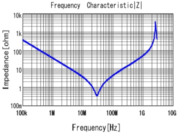
■ DE2E3KY472MN3AM02F |Z| DCOV, 20degC
