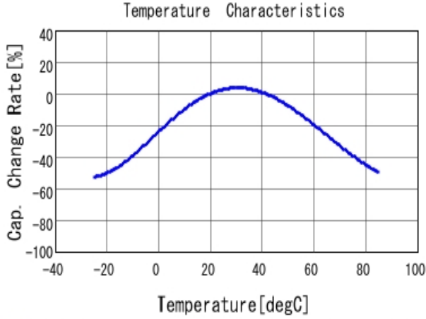
■ DE2E3KY472MN3AM02F C-Temp. capchange, DCOV, AC1Vrms
