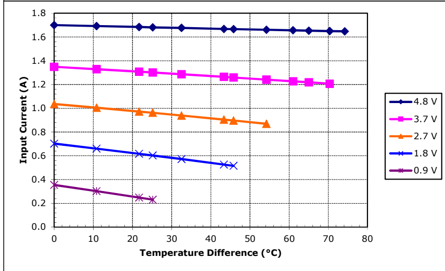
Potted TE-35-0.6-1.0 at a hot-side temperature of 50 °C
