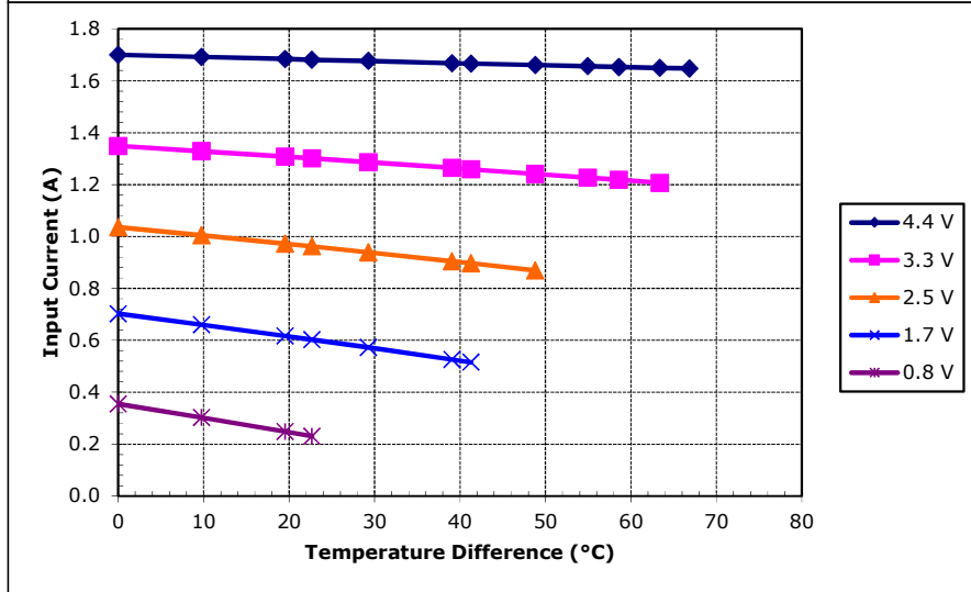
Potted TE-35-0.6-1.0 at a hot-side temperature of 30 °C
