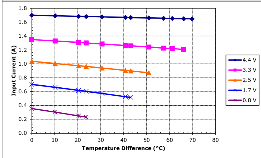
Unpotted TE-35-0.6-1.0 at a hot-side temperature of 30 °C
