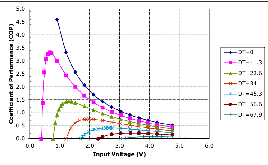
Unpotted TE-35-0.6-1.0 at a hot-side temperature of 50 °C
