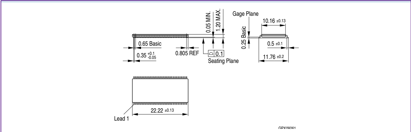
Package Outline of P-TSOPII-66-1 (non-green/green)
