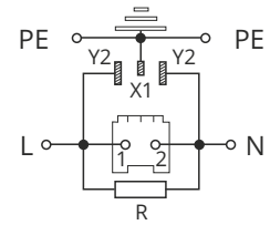
ELECTRICAL CONNECTION
