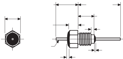
# 4- 40 UNC - 2A Thread Miniature Bushing
