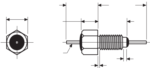
# 4- 40 UNC - 2A Thread Standard Bushing
