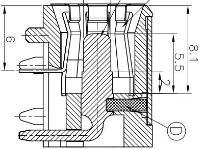
Ø5.50 PLUG TYPE(2DP-G213-BG6) RATING: DC 30V 10A 44uF
