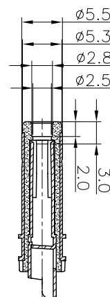
Ø5.50 PLUG TYPE(2DP-G213-BG6) RATING: DC 30V 10A 44uF
