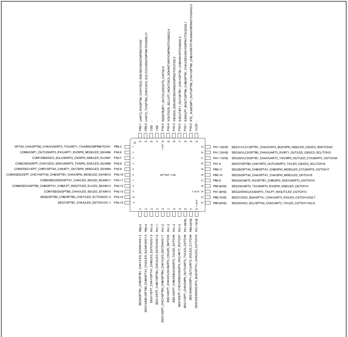
Figure 2-2 管脚定义图(44 QFP)
