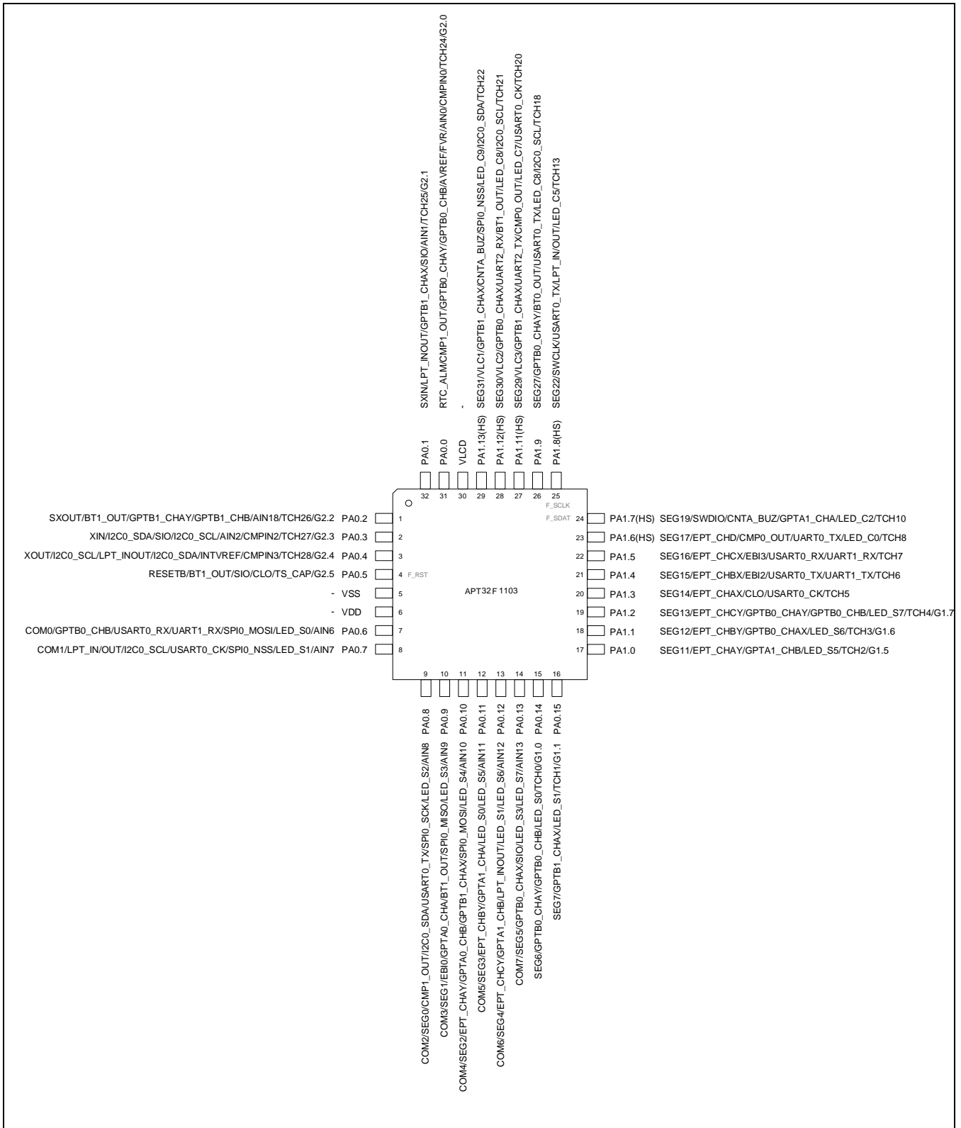
Figure 2-3 管脚定义图(32 LQFP/32 QFN)
