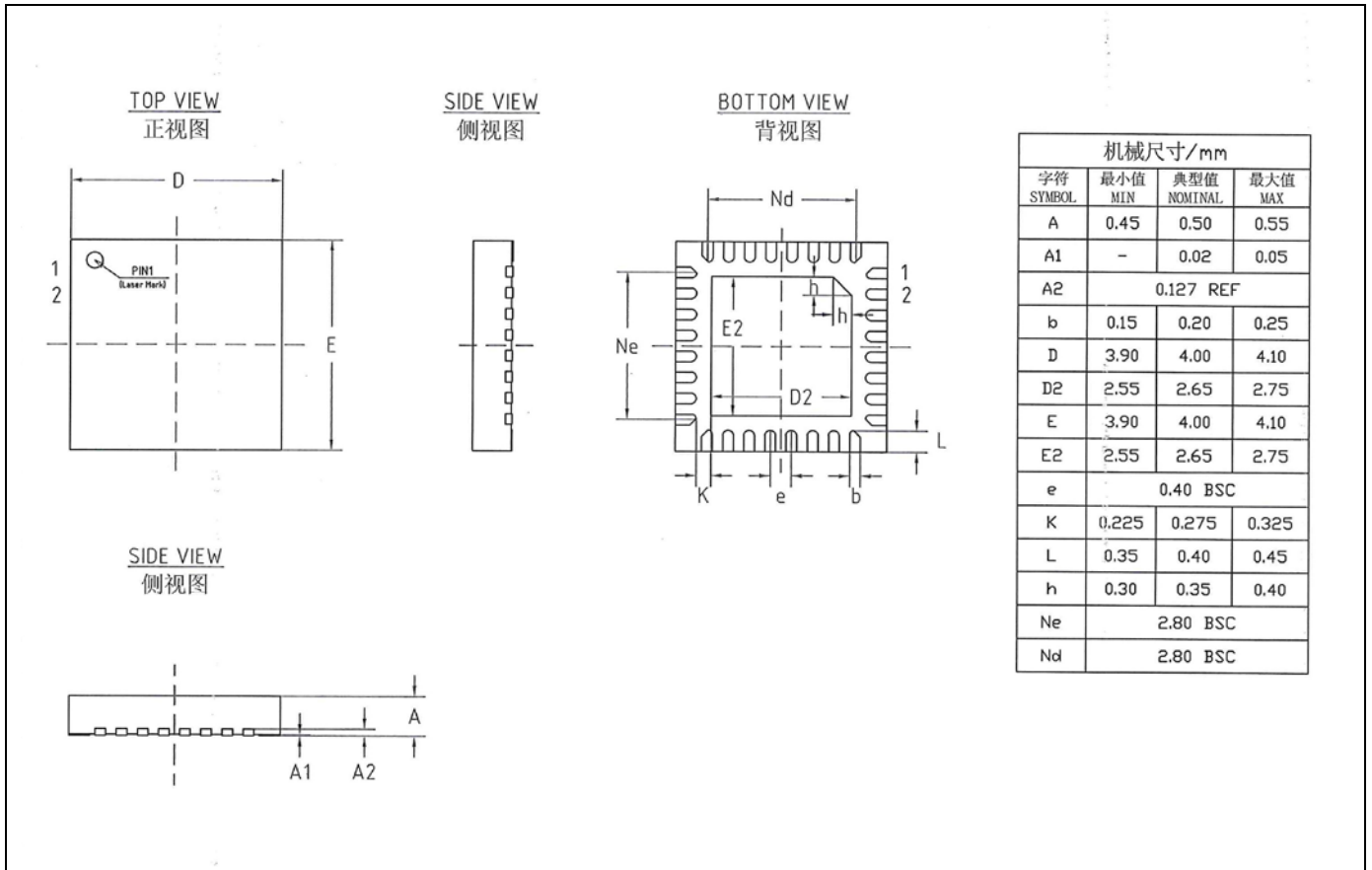
Figure 4-5 QFN32 (4x4-P0.4mm)封装尺寸
