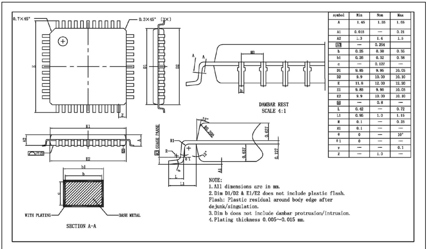
Figure 4-3 44-QFP (10x10-P0.8mm) 封装尺寸
