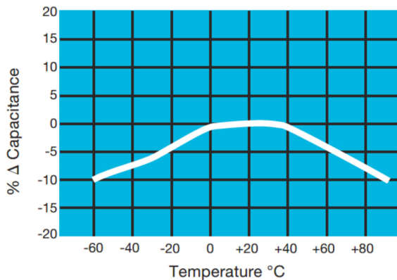
Temperature Coefficient
