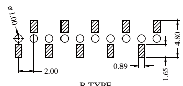
Recommended P.C.B Layout(Bottom Enter) (PCB BOARD TOLERANCE±0.05)
