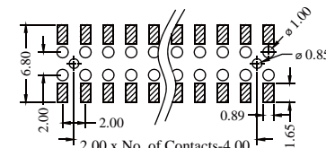
Recommended P.C.B Layout(Bottom Enter) (PCB BOARD TOLERANCE±0.05)
