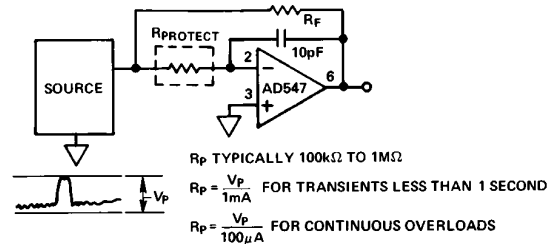
Figure 30. Input Protection
