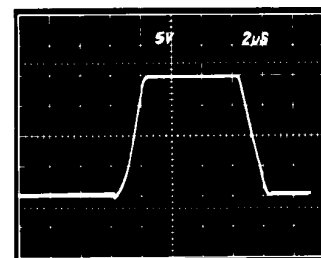
Figure 28. Transient Response R L = 2 kΩ C L = 500 pF—AD544
