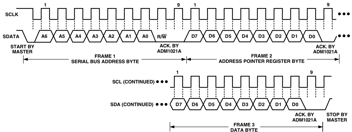
Figure 3. Writing a Register Address to the Address Pointer Register, then Writing Data to the Selected Register
