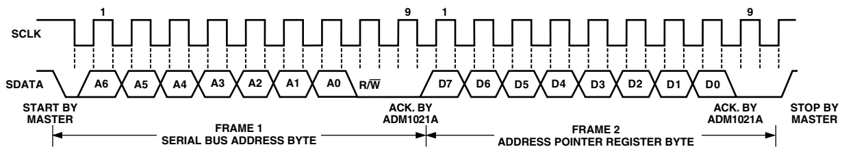
Figure 4. Writing to the Address Pointer Register Only
