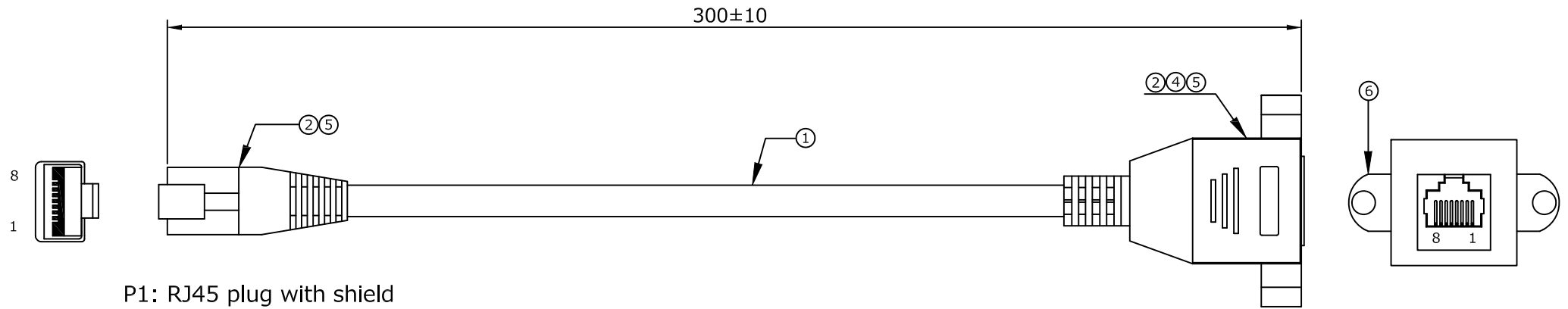
P2: RJ45 socket
