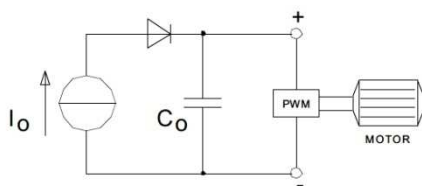
Conventional power supply: breaking power charges output capacitor C_o
