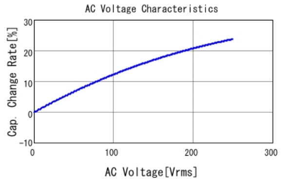
■ DE1E3KX332MA4BN01F C-AC Voltage capchange, DCOV, 20.0
