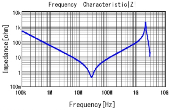
■ DE1E3KX332MA4BN01F |Z| DCOV, 20degC
