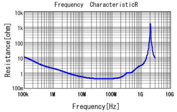
■ DE1E3KX332MA4BN01F R DCOV, 20degC
