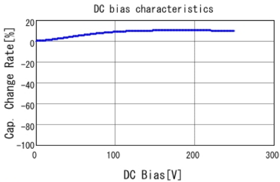
■ DE1E3KX332MA4BN01F C-DC bias capchange, 20.0degC, AC1
