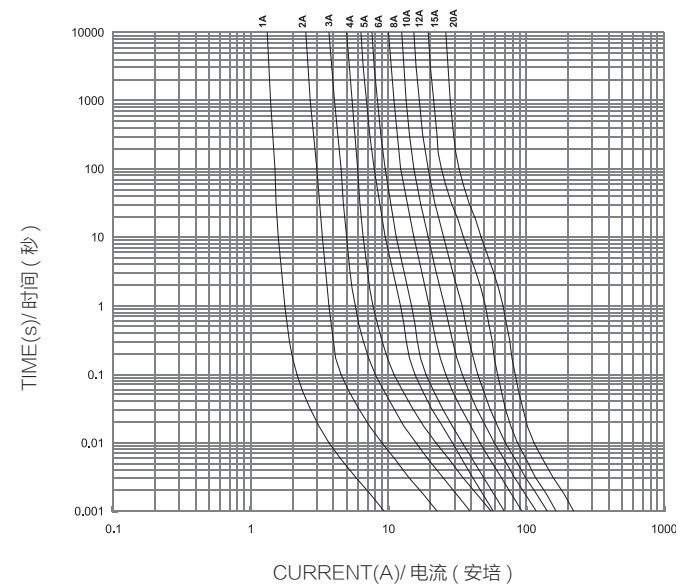
AVERAGE I-T CHARACTERISTICS CURVE (FOR REFERENCE ONLY)
