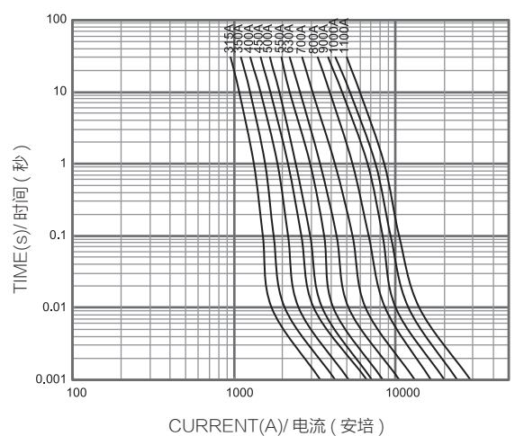
H3BF 平均 I-T 曲线图 (仅供参考) AVERAGE I-T CHARACTERISTICS CURVE (FOR REFERENCE ONLY)
