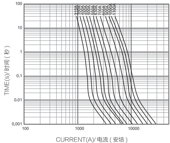
H3BF 平均 I-T 曲线图 (仅供参考) AVERAGE I-T CHARACTERISTICS CURVE (FOR REFERENCE ONLY)
