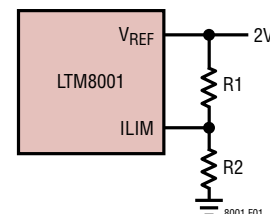
Figure 1. Setting the Output Current Limit, I MAX
