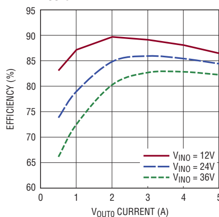
Efficiency vs Output Current, V_{OUT0} = 3.3\text{V}
