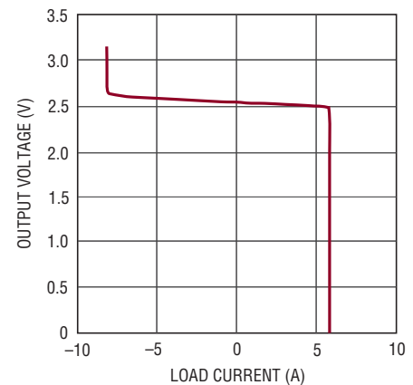
Output Voltage vs Output Current, V_{\text{OUTO}} = 2.5\text{V}
