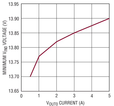
Minimum V_{\text{INO}} vs Output Current, V_{\text{OUTO}} = 12\text{V}
