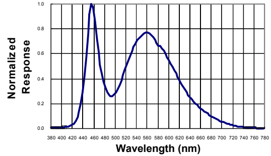
Spectral Radiance
