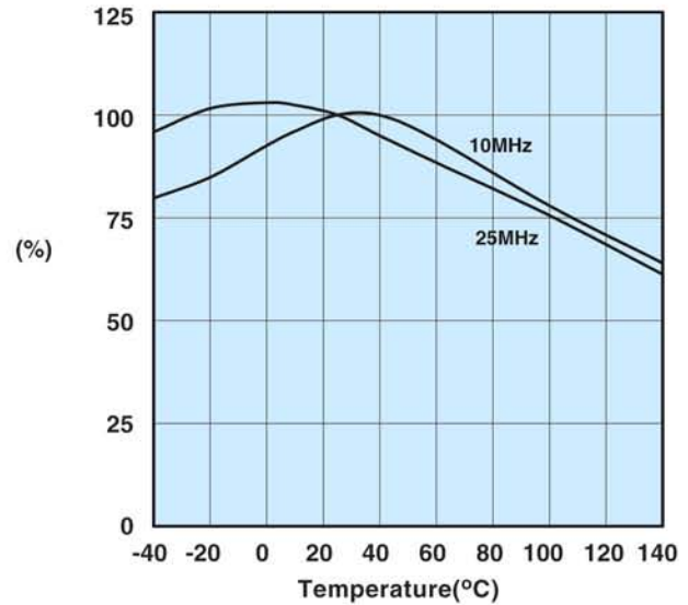
Figure 12 Percent of Original Impedance vs. Temperature Measured on a 2673000301 using the HP4291A.
