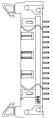
2216S-64G-XX-XX-XX-H
