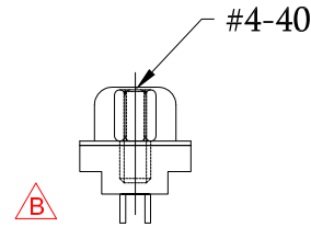
57DBDSXM-XXNCXXXXA-A1 Thread Insert #4-40 +Jack Screw #4-40 Removable
