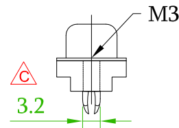
57DBDSXM-XXBOXXXA-A1 With Boardlock Thread Insert M3
