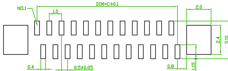
Recommended PCB Board Hole Layout
