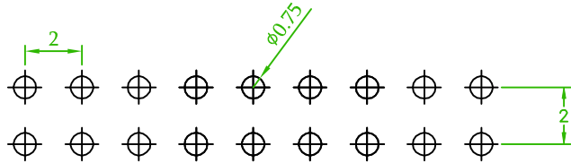
Recommended PCB Layout (PCB TOLERANCE ±0.1)
