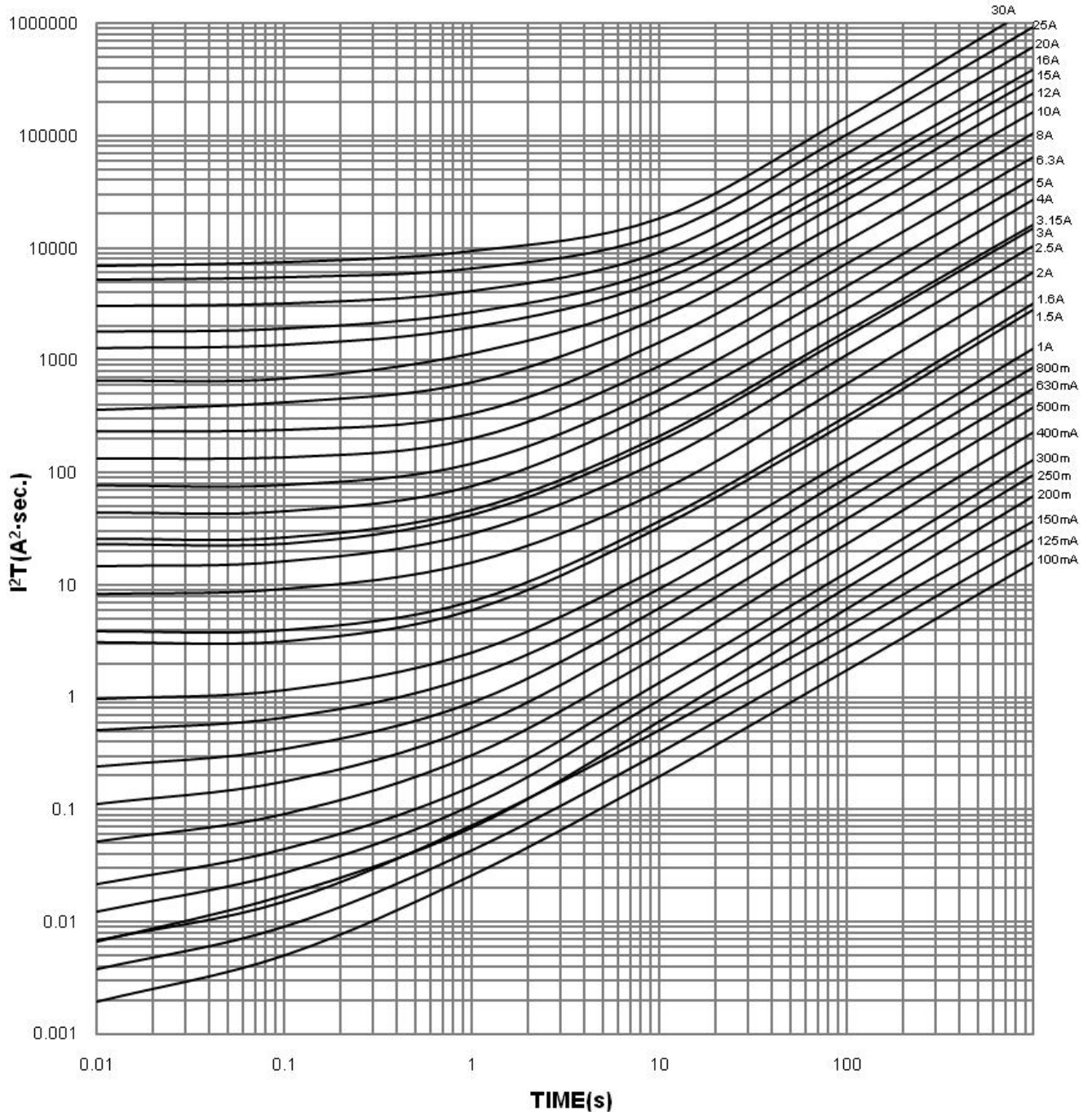
61NM RoHS Average I 2 T-T Characteristics Curve(For Reference Only)
