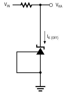
Figure 1c. Test Circuit 3
