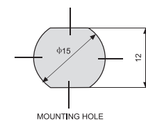
HF-009 PANEL MOUNT FUSE HOLDER FOR 6x32MM FUSE
