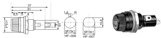
HF-006 HF-007 PANEL MOUNT FUSE HOLDER FOR 5x20MM FUSE
