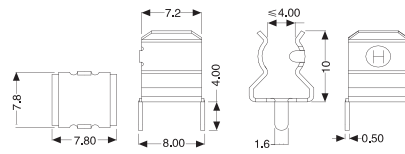
HF-005/N (NICKEL PLATED) (RoHS) HF-005/T (TIN PLATED) (RoHS) FUSE CLIP FOR 6x32MM FUSE
