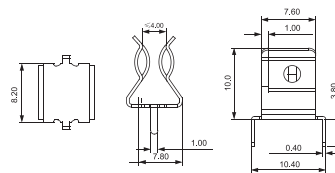
HF-005/I (RoHS) FUSE CLIP FOR 6x32MM FUSE NICKEL PLATED OR TIN PLATED
