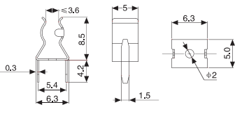
HF-004/D (RoHS) FUSE CLIP FOR 5x20MM FUSE NICKEL PLATED OR TIN PLATED
