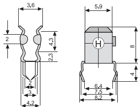
HF-004/J (RoHS) FUSE CLIP FOR 5x20MM FUSE NICKEL PLATED OR TIN PLATED
