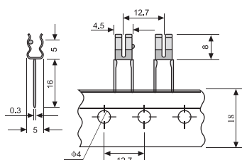
HF-004/PT (RoHS) FUSE CLIP FOR 5x20MM FUSE, TAPED TYPE PHOSPHOR BRONZE, TIN PLATED
