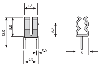
HF-004/PT (RoHS) FUSE CLIP FOR 5x20MM FUSE, TAPED TYPE PHOSPHOR BRONZE, TIN PLATED
