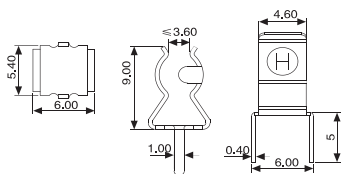
HF-004/P (RoHS) FUSE CLIP FOR 5x20MM FUSE PHOSPHOR BRONZE, TIN PLATED
