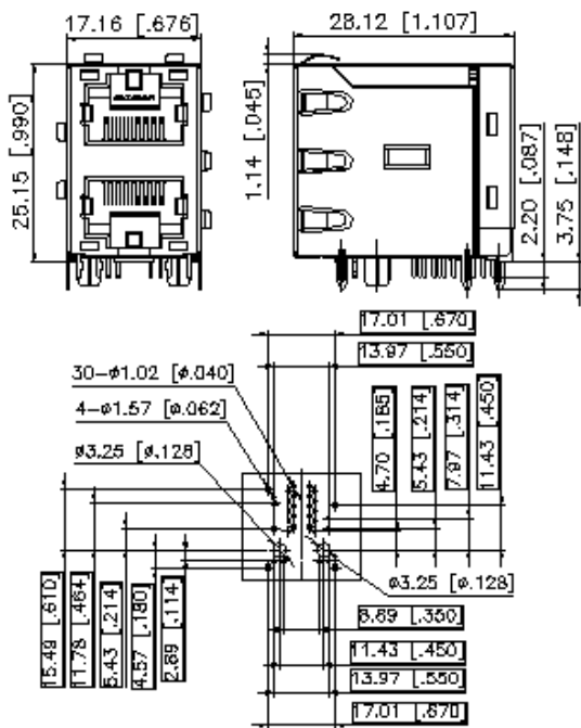
RECOMMENDED PRINTED CIRCUIT BOARD LAYOUT TOP VIEW (COMPONENT SIDE)
