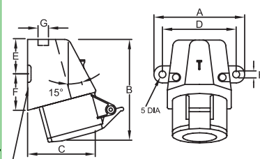
BLIND KNOCKOUT FOR REAR CABLE ENTRY 20/25mm
