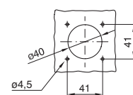
Drilling template
