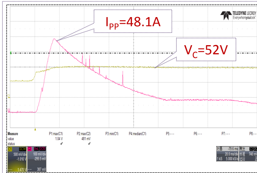
Test Rule: ISO16750-2 5a Test R_i=3\Omega
