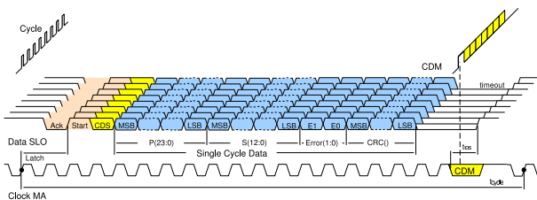
Figure 17: Example line signals (BiSS C)
