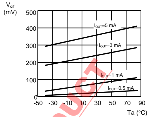
7.2 S-81215SG series
