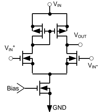
Figure 5 Error amplifier
