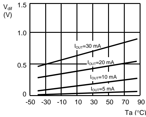
7.9 S-81250SG series
