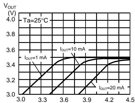
1.8 S-81245SG series
