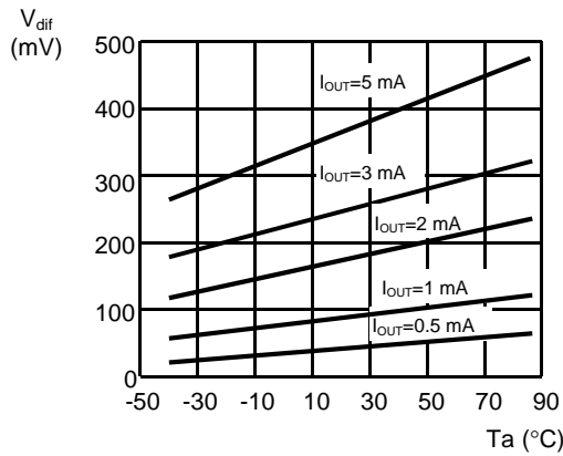
7.1 S-81211SG series
