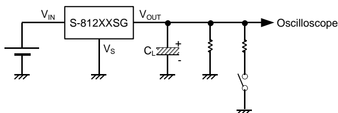
Figure 10 Measuring circuit
