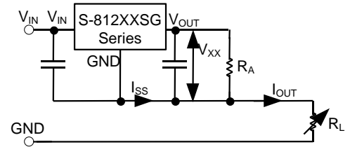
Figure 16 Constant current regulator
