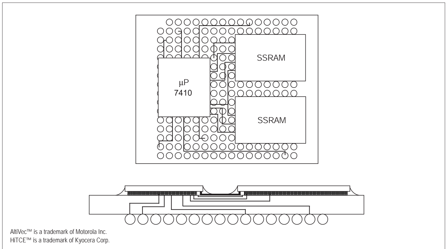
FIGURE 1 – MULTI-CHIP PACKAGE DIAGRAM
