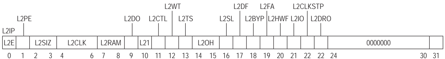
FIGURE 5 – L2 CACHE CONTROL REGISTER (L2CR)
