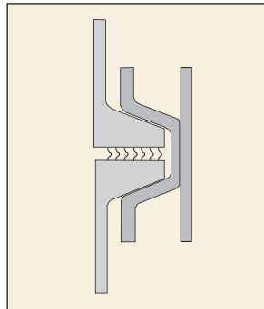
Style MC
