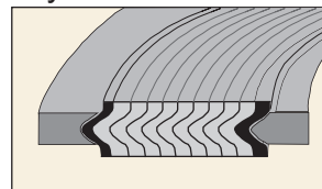
Style CGI
