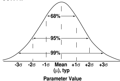
Figure 10. Normal Distribution.
