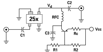
Figure 4. Active Bias Circuit.
