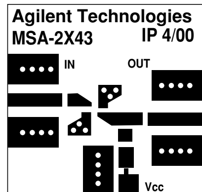
Figure 3. Multi-purpose Evaluation Board.
