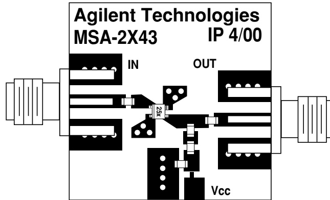
Figure 6. Complete 1.9 GHz Amplifier.
