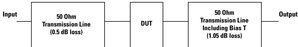
Block diagram of 2 GHz production test board used for gain measurements. Circuit losses have been de-embedded from actual measurements.
