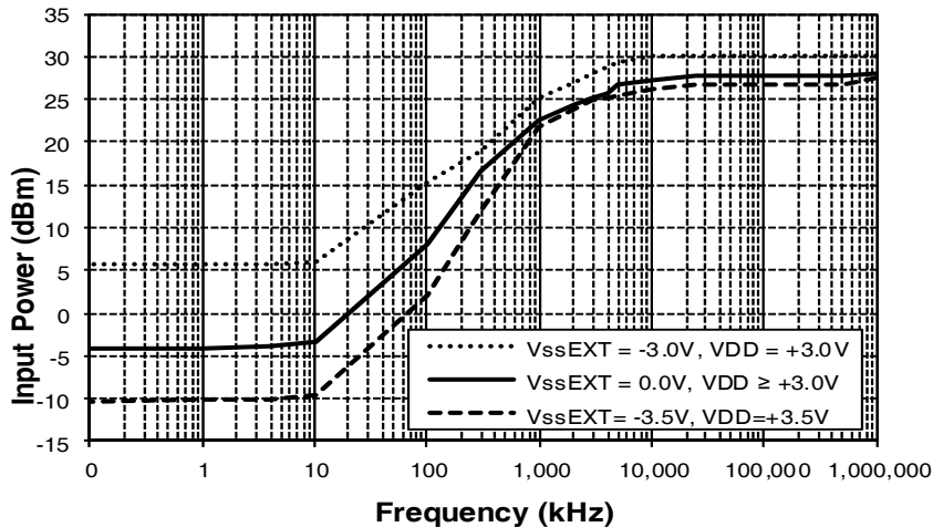
Figure 6. Maximum Operating Power vs Frequency ( T_{\text{ambient}} = +85\text{ }^{\circ}\text{C} )
