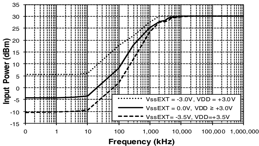
Figure 5. Maximum Operating Power vs Frequency ( T_{\text{ambient}} = +50\text{ }^{\circ}\text{C} )
