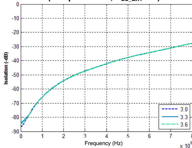
Figure 12. Isolation: RFX-RFC vs V_{DD} (Temp = +25°C, V_{SS\_EXT} = 0 )
