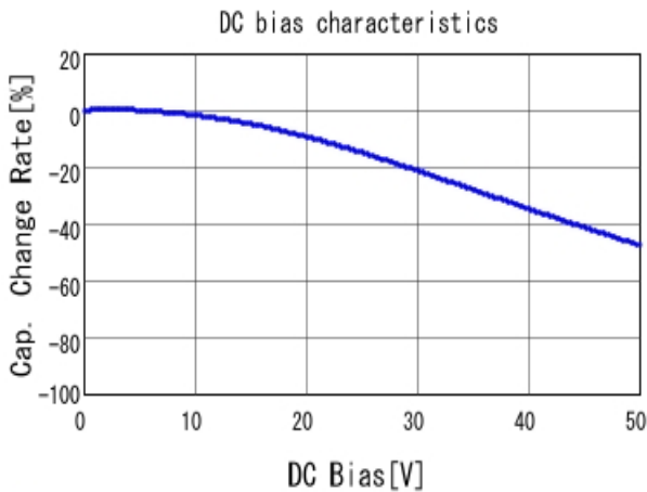
■ GRM155B31H682KA88 C-DC bias capchange, 20.0degC, AC1.
