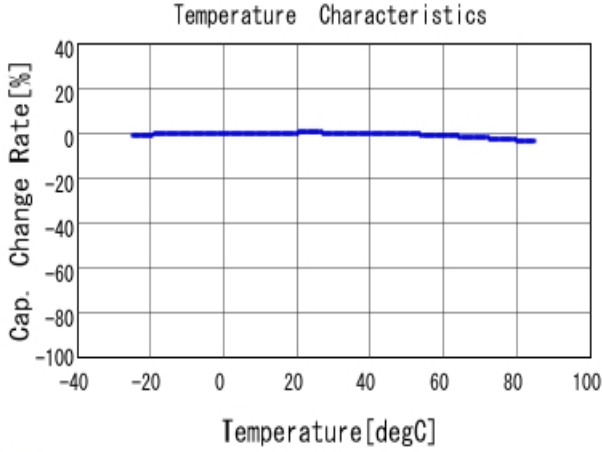
■ GRM155B31H682KA88 C-Temp. capchange, DCO. 0V, AC1.0V rm
