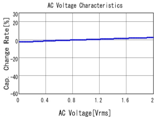
■ GRM155B31H682KA88 C-AC Voltage capchange, DCOV, 20.0d
