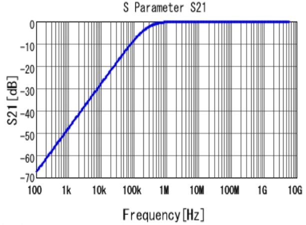
■ GRM155B31H682KA88 S21 DCOV, 20degC
