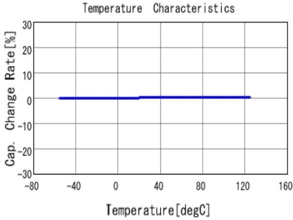
■ GRM1882C1H8R0DA01 C-Temp. capchange, DCOV, AC1Vrms
