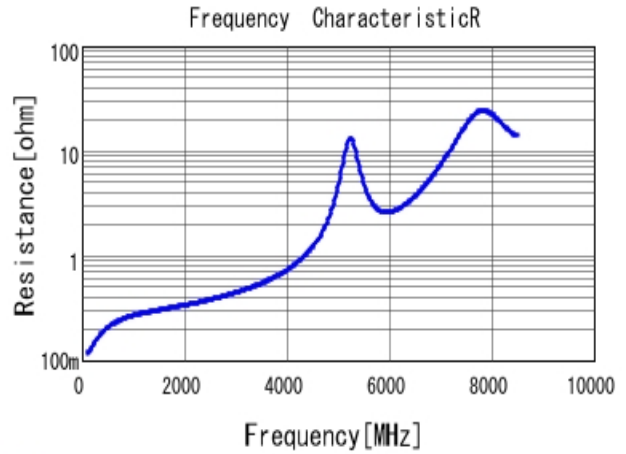
■ GRM1882C1H8R0DA01 R DCOV, 20degC
