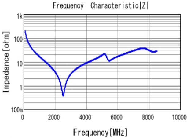
■ GRM1882C1H8R0DA01 |Z| DCOV, 20degC
