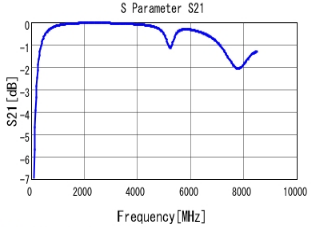
■ GRM1882C1H8R0DA01 S21 DCOV, 20degC
