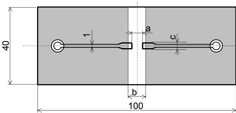
RMC1/2, 1 TERMINAL STRENGTH TEST SUBSTRATE
