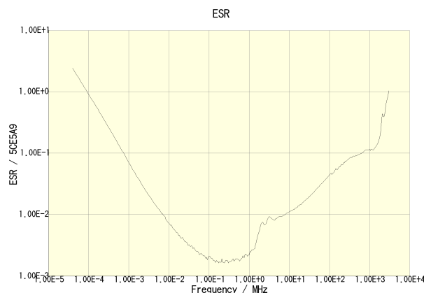
C3225X5R0J226M200AA
