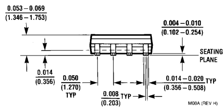
Molded Package, Small Outline, 0.15 Wide, 8-Lead (M8) NS Package Number M08A
