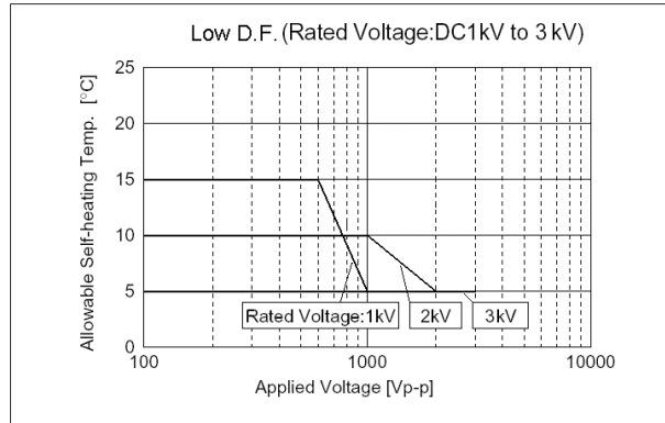
Fig 2: Dependence of Self-heating Temperature on Ambient Temperature
