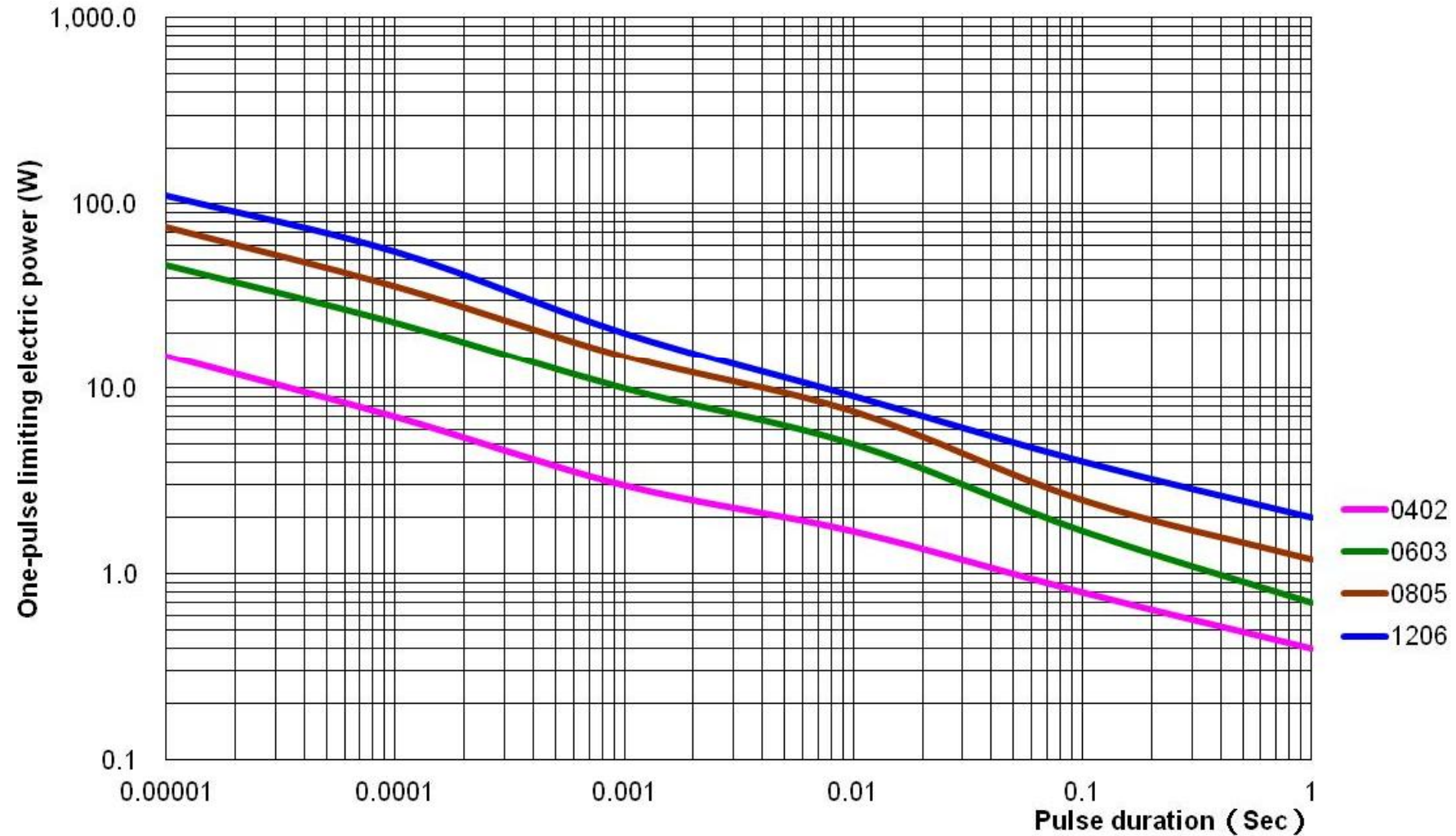
Maximum permissible peak pulse power as a function of pulse duration
