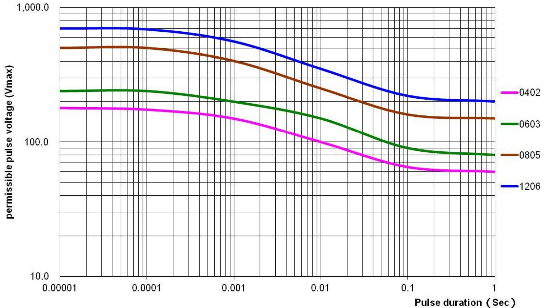
Maximum permissible peak pulse voltage as a function of pulse duration
